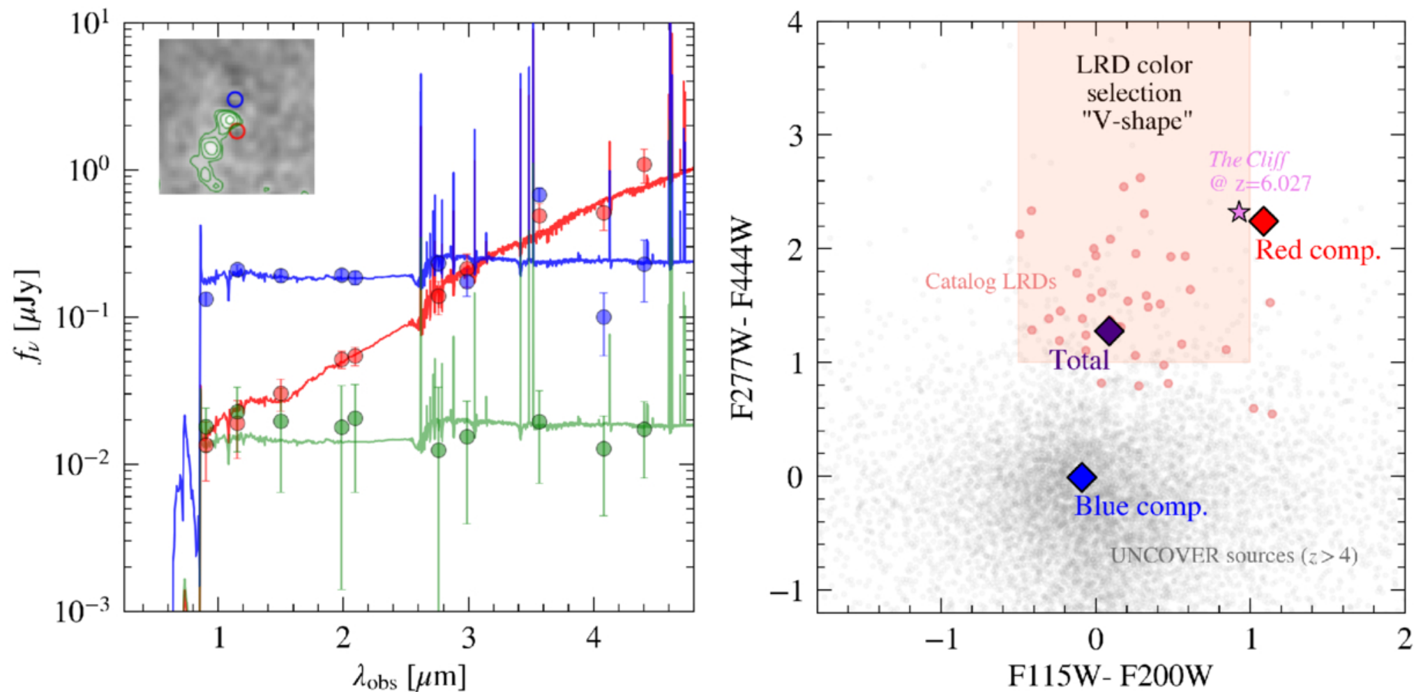
Figure 5. from Josephine F. W. Baggen et al 2026 Astrophys. J. Lett. 1006 doi:10.3847/2041-8213/ae82fe https://dx.doi.org/10.3847/2041-8213/ae82fe © 2026. The Author(s). Published by the American Astronomical Society.
