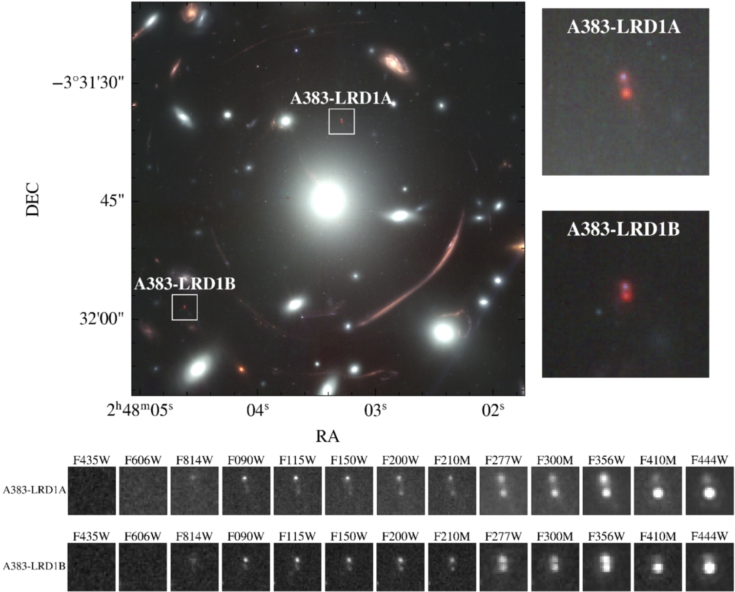
Figure 1. from Josephine F. W. Baggen et al 2026 Astrophys. J. Lett. 1006 doi:10.3847/2041-8213/ae82fe https://dx.doi.org/10.3847/2041-8213/ae82fe © 2026. The Author(s). Published by the American Astronomical Society.
