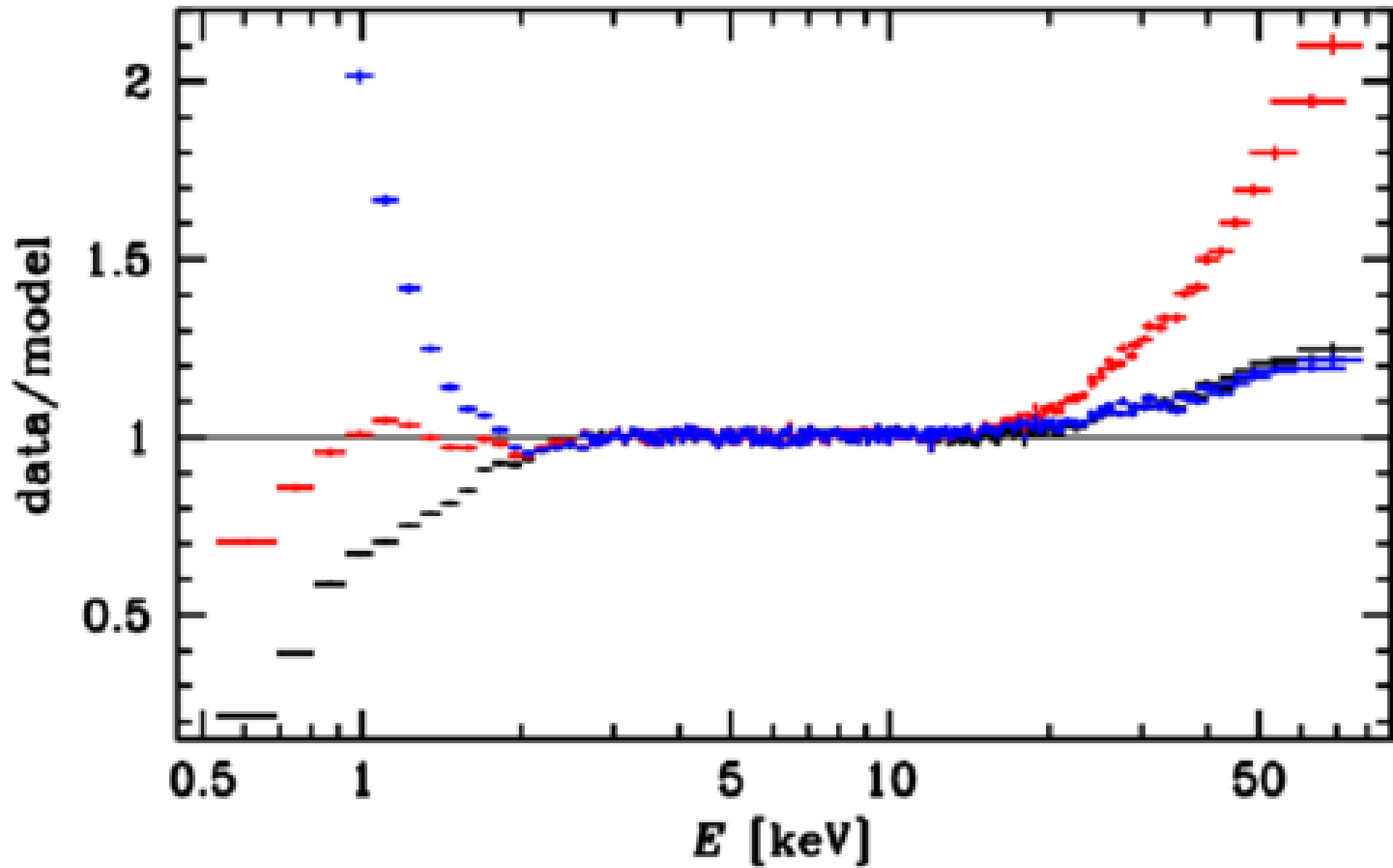
Figure 5. from Andrzej A. Zdziarski et al 2026 Astrophys. J. Lett. 1005 doi:10.3847/2041-8213/ae82fa https://dx.doi.org/10.3847/2041-8213/ae82fa © 2026. The Author(s). Published by the American Astronomical Society.
