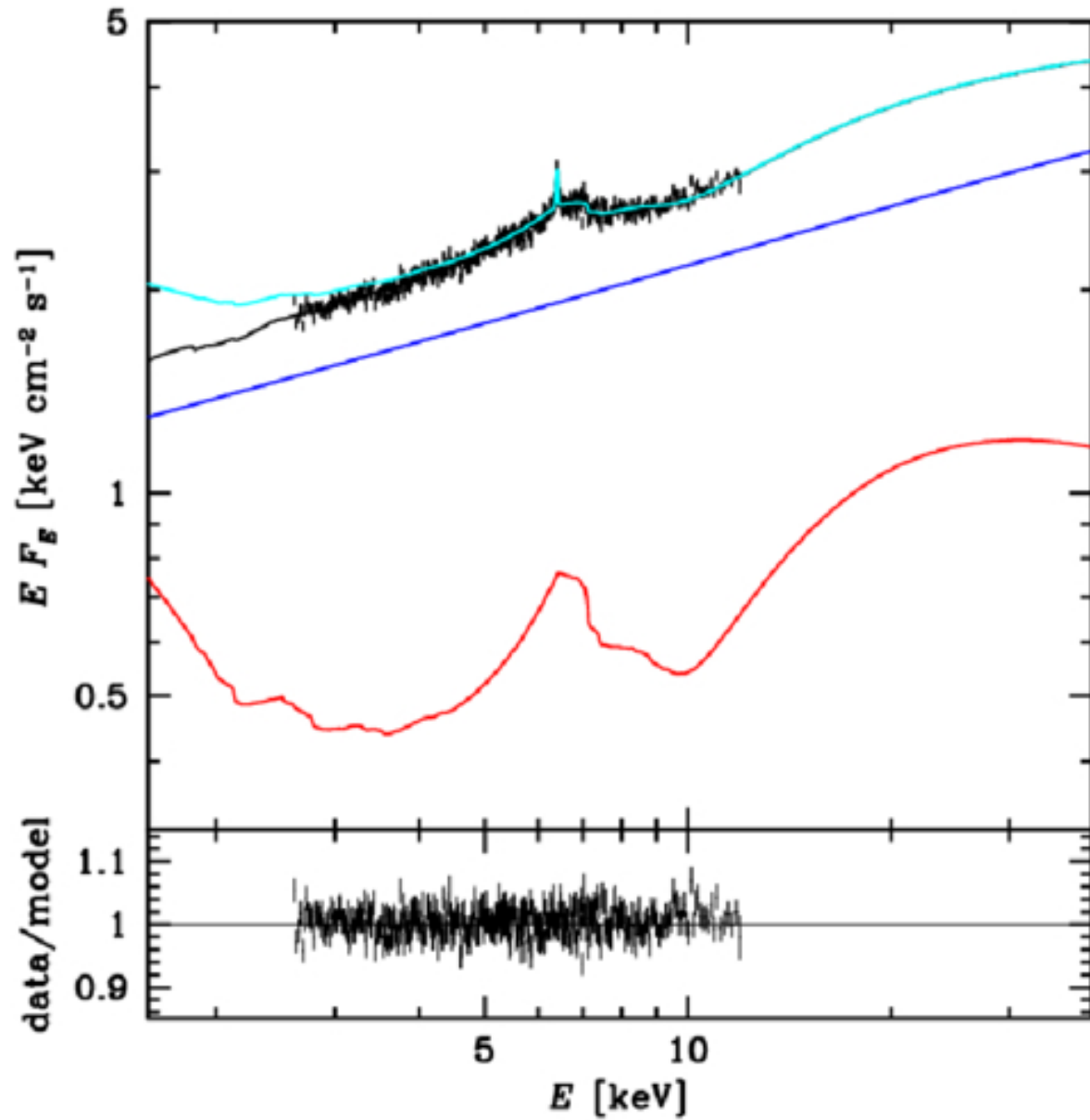
Figure 4. from Andrzej A. Zdziarski et al 2026 Astrophys. J. Lett. 1005 doi:10.3847/2041-8213/ae82fa https://dx.doi.org/10.3847/2041-8213/ae82fa © 2026. The Author(s). Published by the American Astronomical Society.
