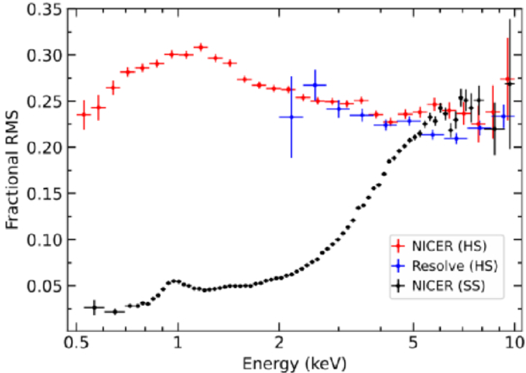
Figure 3. from Andrzej A. Zdziarski et al 2026 Astrophys. J. Lett. 1005 doi:10.3847/2041-8213/ae82fa https://dx.doi.org/10.3847/2041-8213/ae82fa © 2026. The Author(s). Published by the American Astronomical Society.
