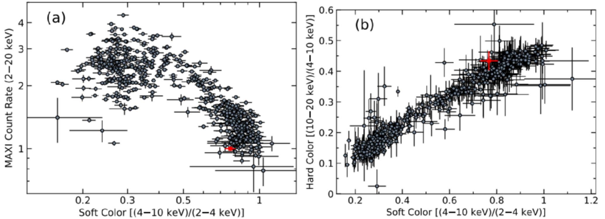
Figure 2. from Andrzej A. Zdziarski et al 2026 Astrophys. J. Lett. 1005 doi:10.3847/2041-8213/ae82fa https://dx.doi.org/10.3847/2041-8213/ae82fa © 2026. The Author(s). Published by the American Astronomical Society.
