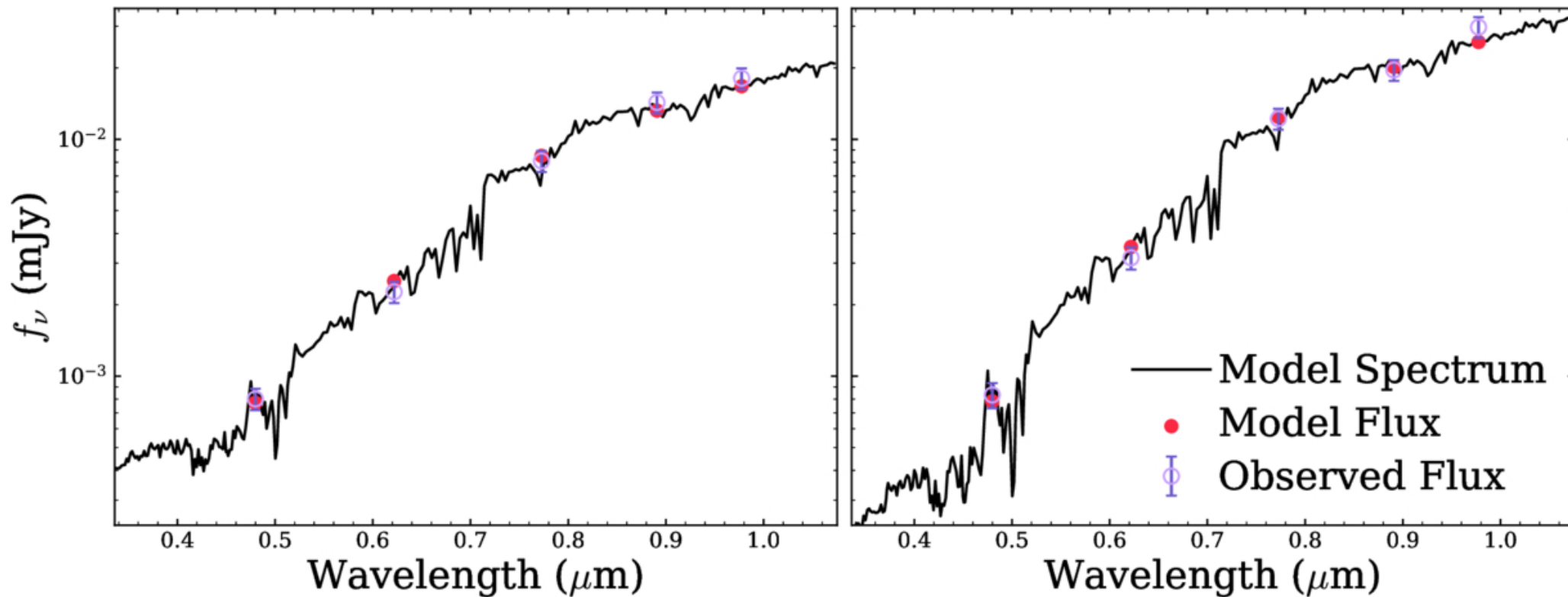
Figure 3. from Zizhao He et al 2026 Astrophys. J. Lett. 1006 doi:10.3847/2041-8213/ae82f9 https://dx.doi.org/10.3847/2041-8213/ae82f9 © 2026. The Author(s). Published by the American Astronomical Society.
