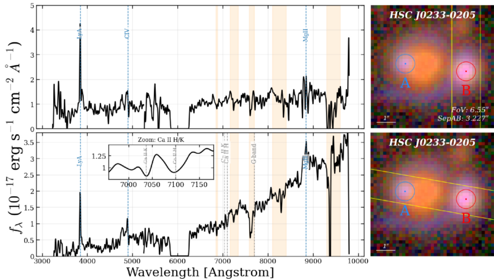
Figure 1. from Zizhao He et al 2026 Astrophys. J. Lett. 1006 doi:10.3847/2041-8213/ae82f9 https://dx.doi.org/10.3847/2041-8213/ae82f9 © 2026. The Author(s). Published by the American Astronomical Society.
