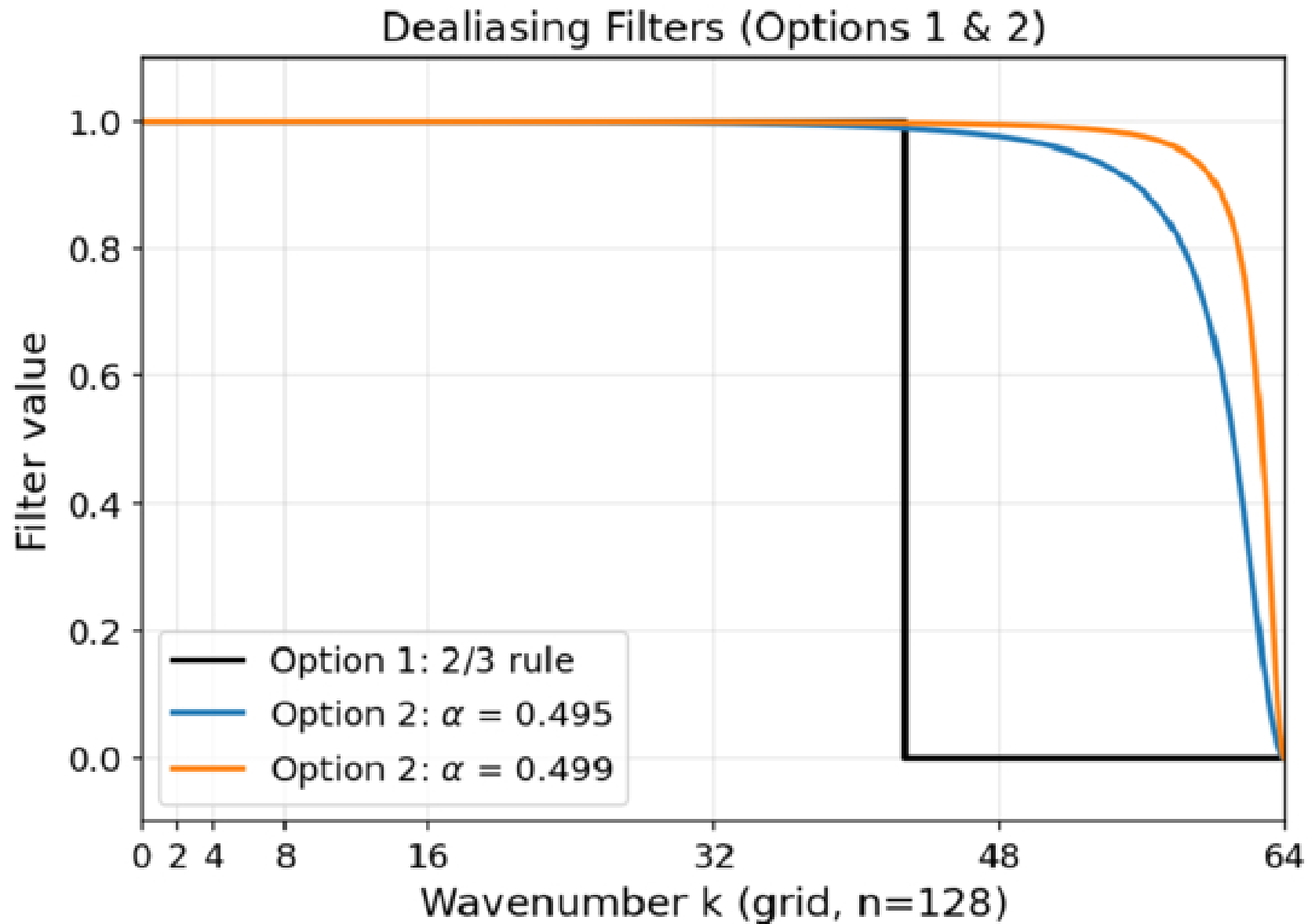
Figure 7. from Zesen Huang et al 2026 Astrophys. J. Lett. 1006 doi:10.3847/2041-8213/ae82f5 https://dx.doi.org/10.3847/2041-8213/ae82f5 © 2026. The Author(s). Published by the American Astronomical Society.
