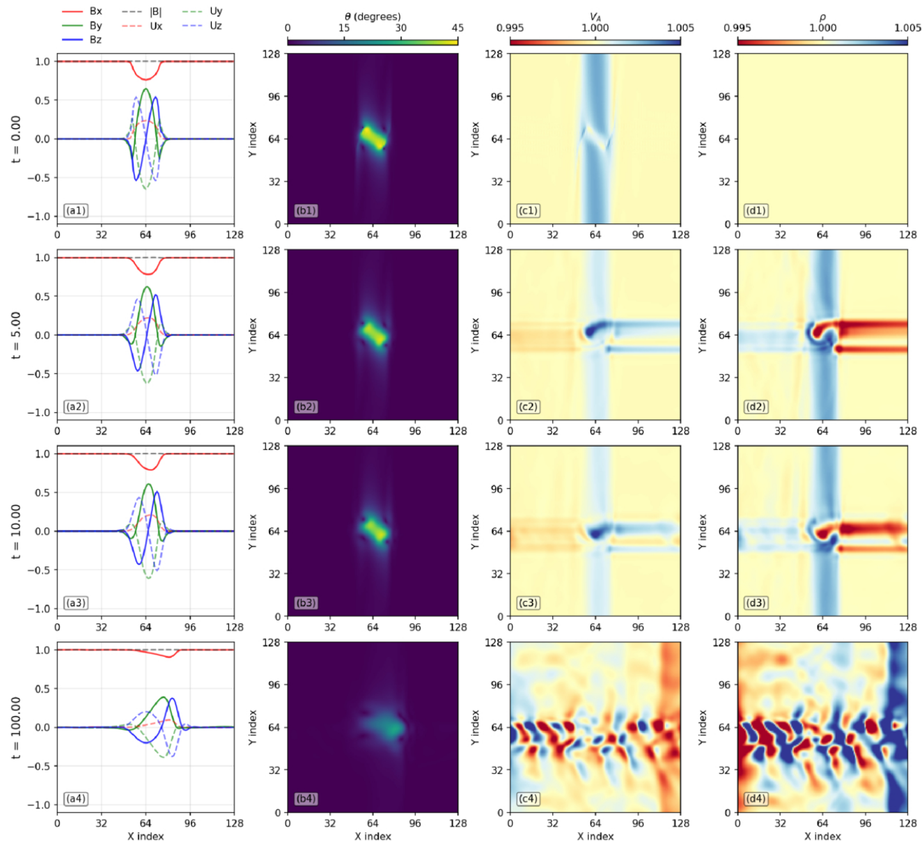
Figure 4. from Zesen Huang et al 2026 Astrophys. J. Lett. 1006 doi:10.3847/2041-8213/ae82f5 https://dx.doi.org/10.3847/2041-8213/ae82f5 © 2026. The Author(s). Published by the American Astronomical Society.
