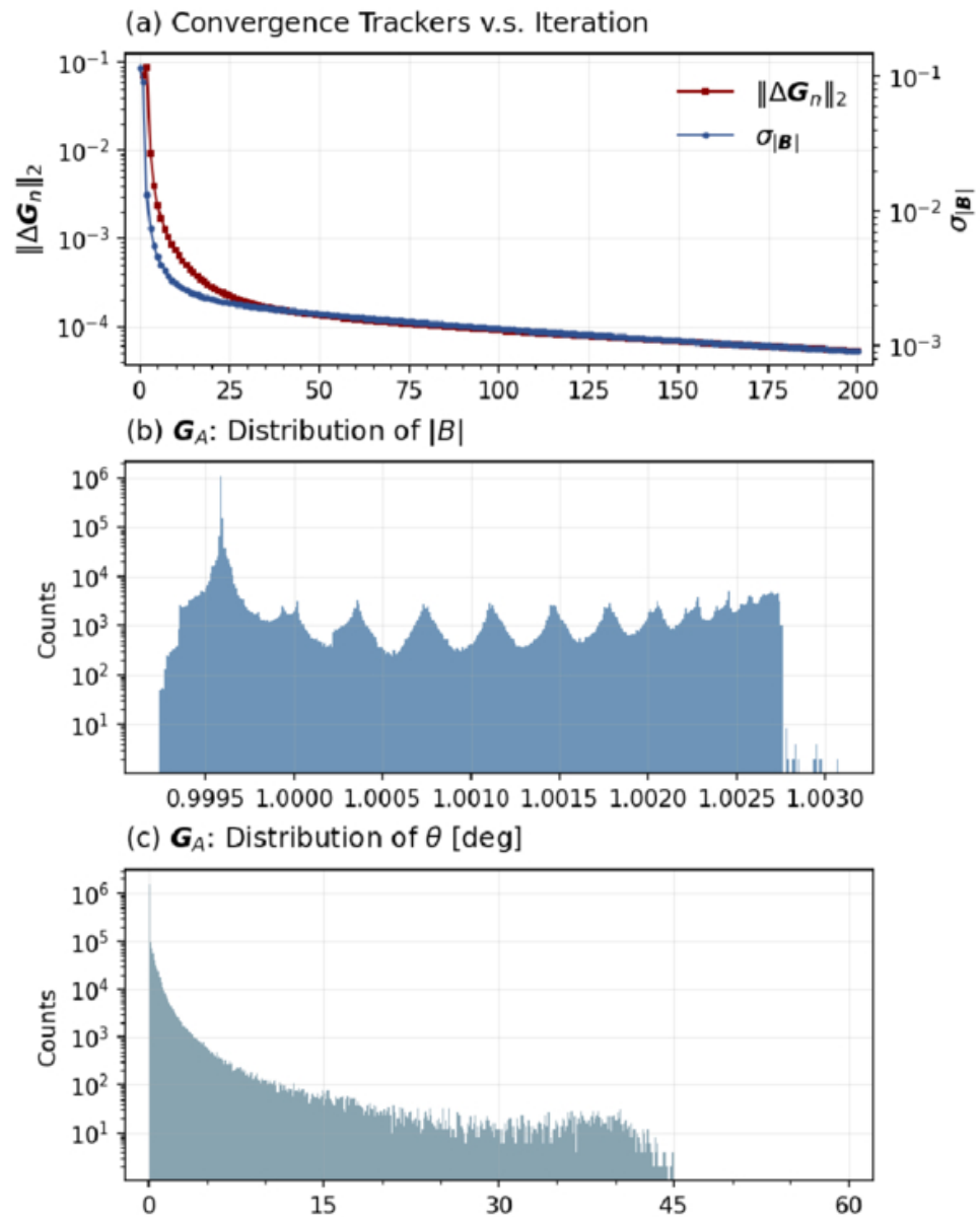
Figure 2. from Zesen Huang et al 2026 Astrophys. J. Lett. 1006 doi:10.3847/2041-8213/ae82f5 https://dx.doi.org/10.3847/2041-8213/ae82f5 © 2026. The Author(s). Published by the American Astronomical Society.
