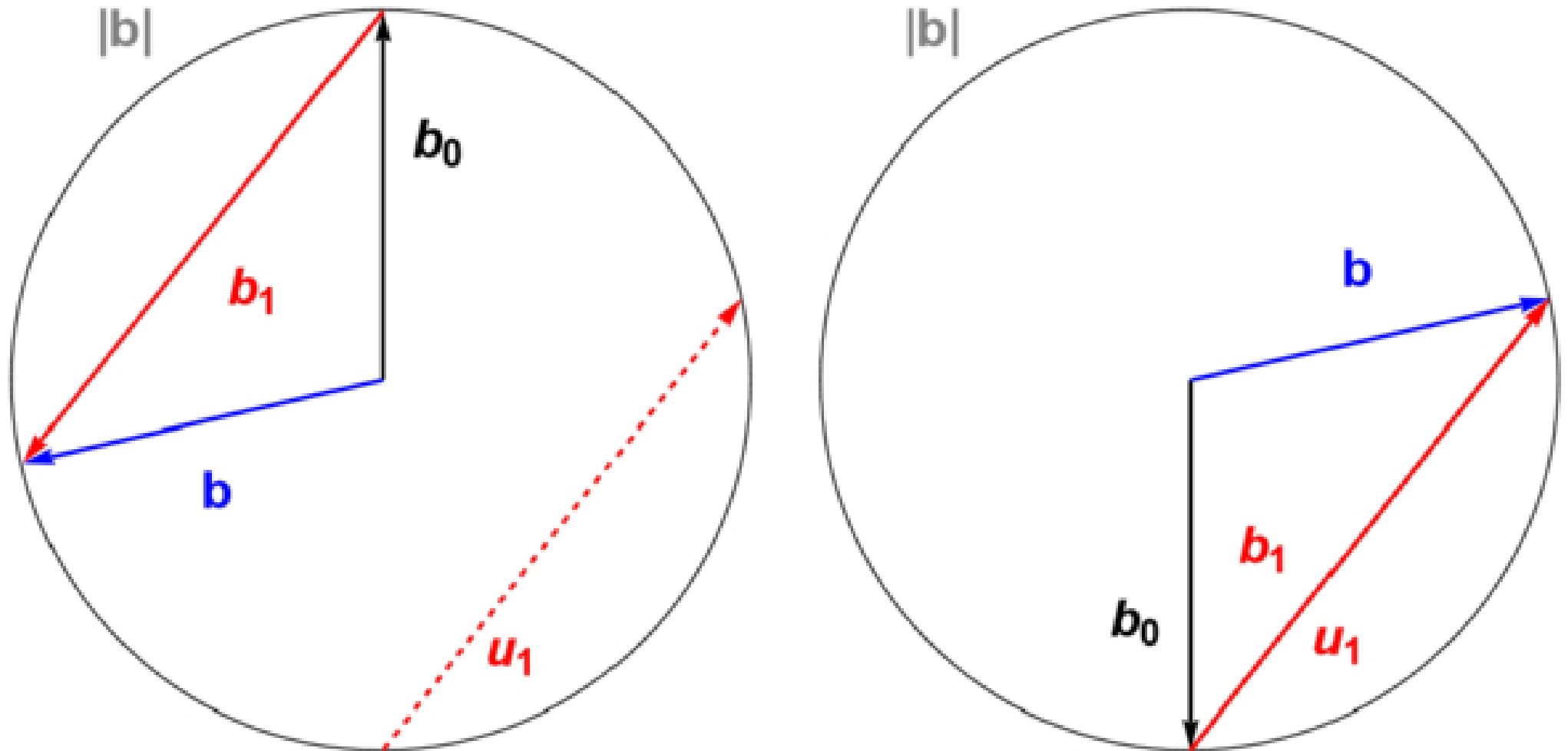
Figure 1. from Zesen Huang et al 2026 Astrophys. J. Lett. 1006 doi:10.3847/2041-8213/ae82f5 https://dx.doi.org/10.3847/2041-8213/ae82f5 © 2026. The Author(s). Published by the American Astronomical Society.
