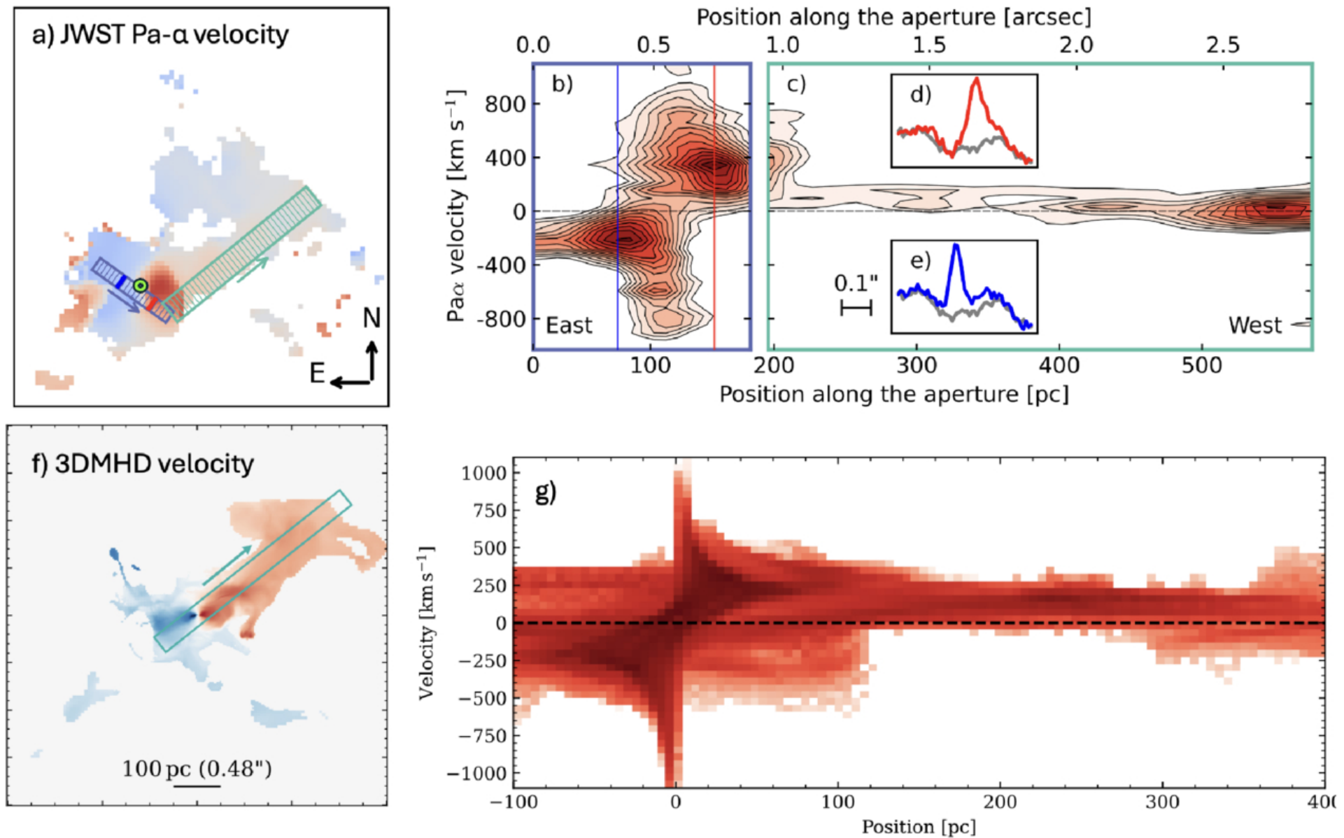
Figure 3. from Julie Hlavacek-Larrondo et al 2026 Astrophys. J. Lett. 1006 doi:10.3847/2041-8213/ae81ae https://dx.doi.org/10.3847/2041-8213/ae81ae © 2026. The Author(s). Published by the American Astronomical Society.
