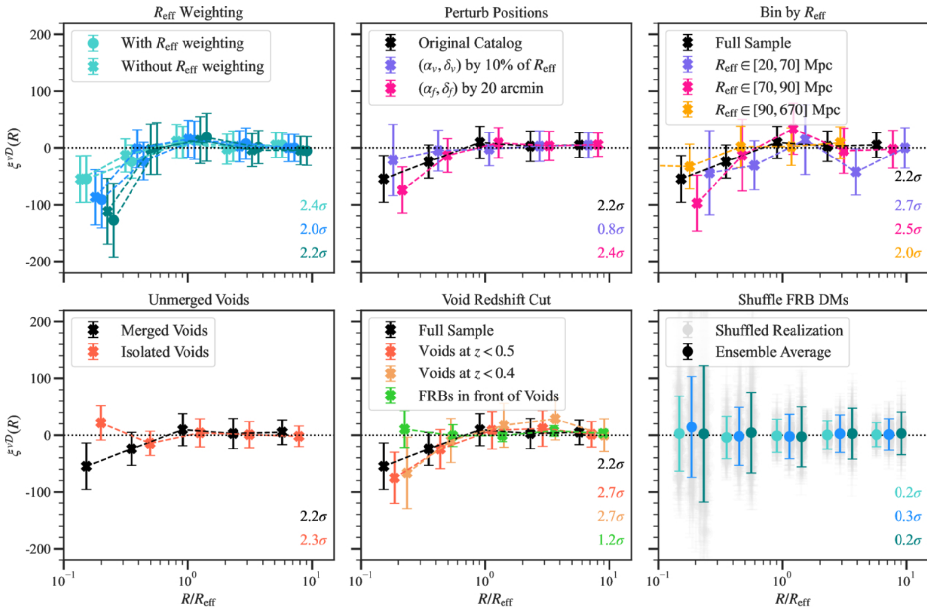
Figure 4. from Kritti Sharma et al 2026 Astrophys. J. Lett. 1006 doi:10.3847/2041-8213/ae81ac https://dx.doi.org/10.3847/2041-8213/ae81ac © 2026. The Author(s). Published by the American Astronomical Society.
