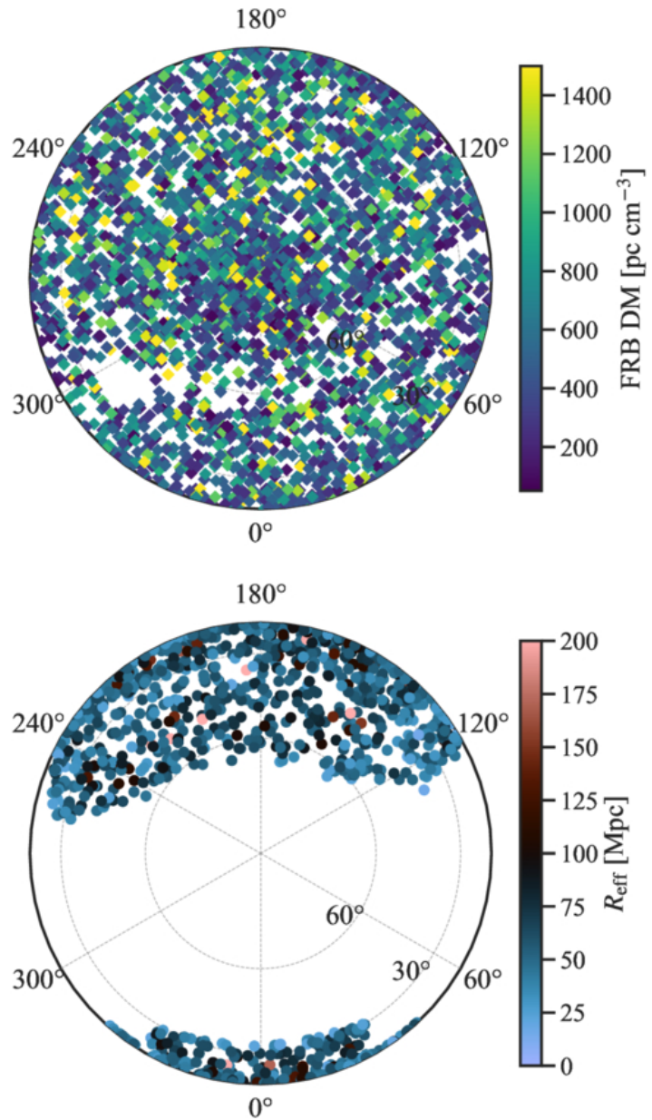
Figure 1. from Kritti Sharma et al 2026 Astrophys. J. Lett. 1006 doi:10.3847/2041-8213/ae81ac https://dx.doi.org/10.3847/2041-8213/ae81ac © 2026. The Author(s). Published by the American Astronomical Society.
