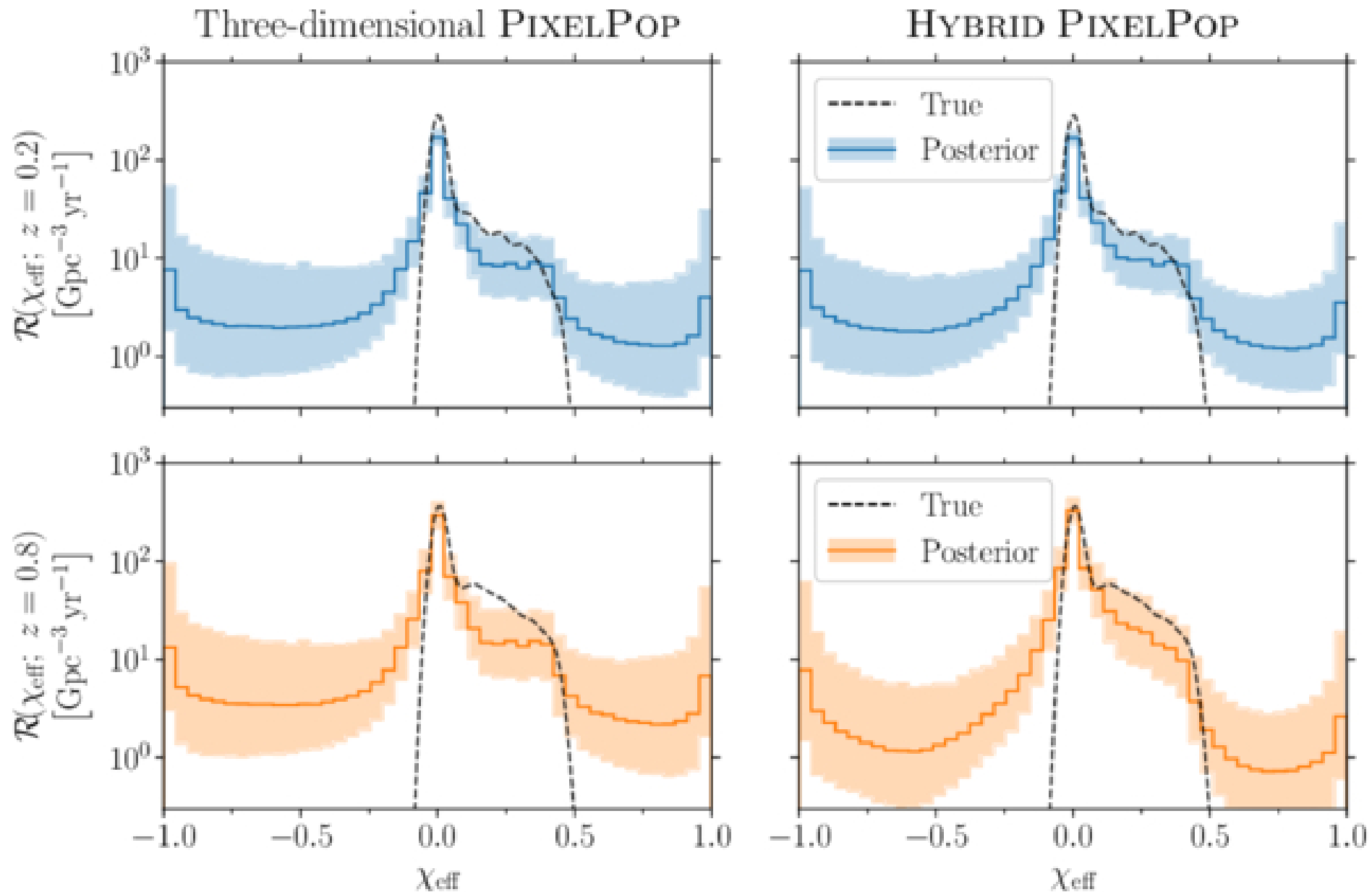
Figure 6. from Sofía Álvarez-López et al 2026 Astrophys. J. Lett. 1006 doi:10.3847/2041-8213/ae81a9 https://dx.doi.org/10.3847/2041-8213/ae81a9 © 2026. The Author(s). Published by the American Astronomical Society.
