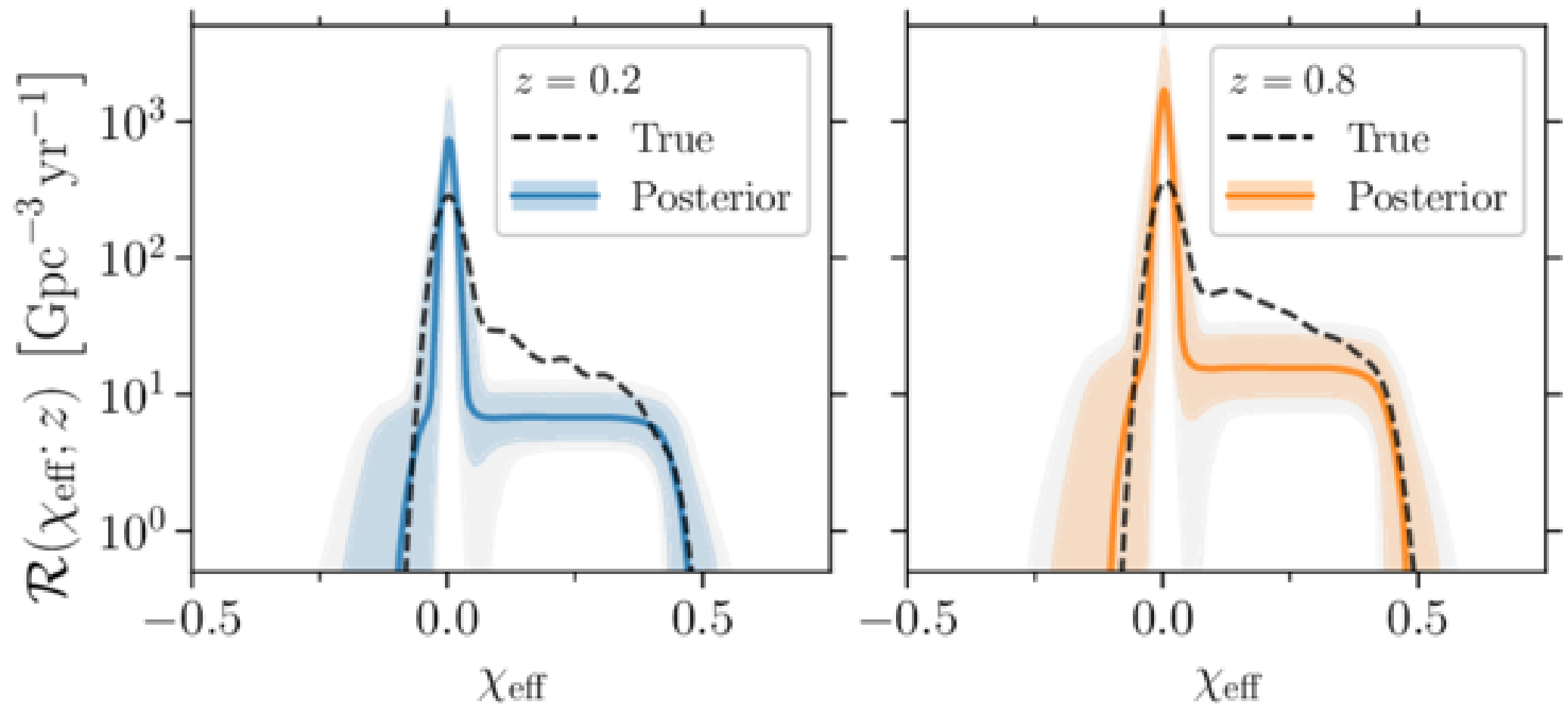
Figure 4. from Sofía Álvarez-López et al 2026 Astrophys. J. Lett. 1006 doi:10.3847/2041-8213/ae81a9 https://dx.doi.org/10.3847/2041-8213/ae81a9 © 2026. The Author(s). Published by the American Astronomical Society.
