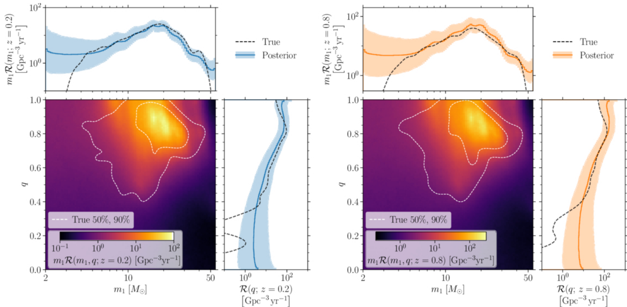
Figure 3. from Sofía Álvarez-López et al 2026 Astrophys. J. Lett. 1006 doi:10.3847/2041-8213/ae81a9 https://dx.doi.org/10.3847/2041-8213/ae81a9 © 2026. The Author(s). Published by the American Astronomical Society.
