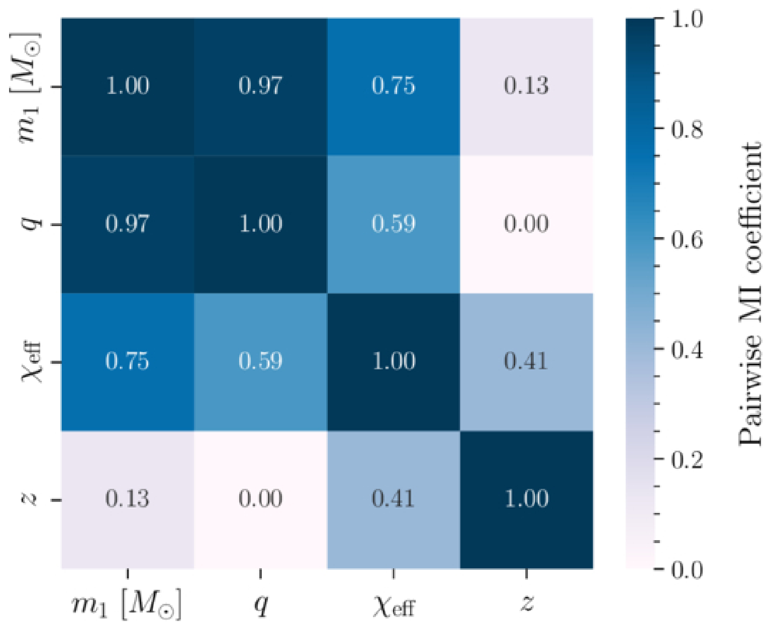
Figure 2. from Sofía Álvarez-López et al 2026 Astrophys. J. Lett. 1006 doi:10.3847/2041-8213/ae81a9 https://dx.doi.org/10.3847/2041-8213/ae81a9 © 2026. The Author(s). Published by the American Astronomical Society.
