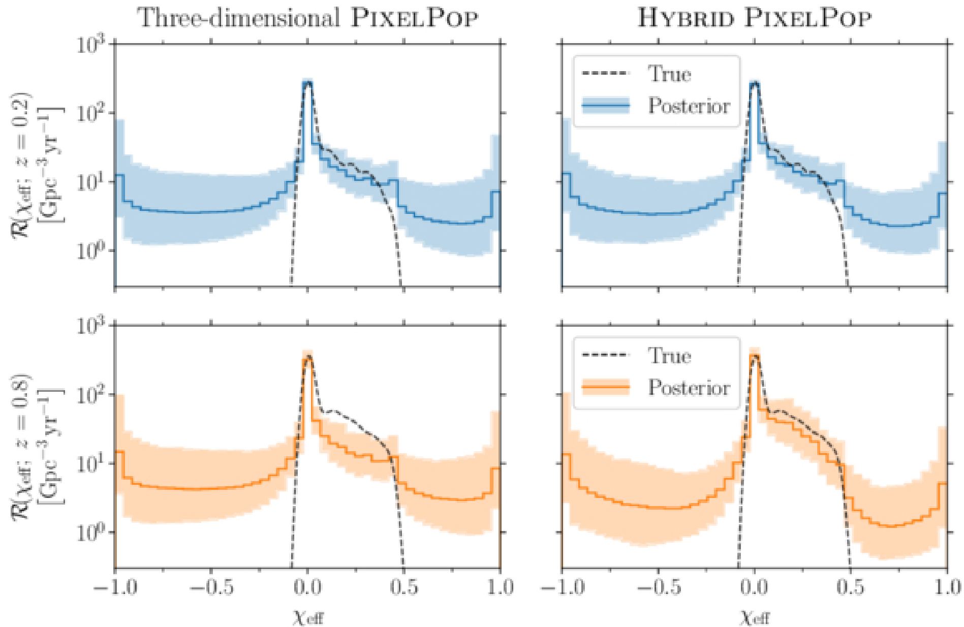
Figure 13. from Sofía Álvarez-López et al 2026 Astrophys. J. Lett. 1006 doi:10.3847/2041-8213/ae81a9 https://dx.doi.org/10.3847/2041-8213/ae81a9 © 2026. The Author(s). Published by the American Astronomical Society.
