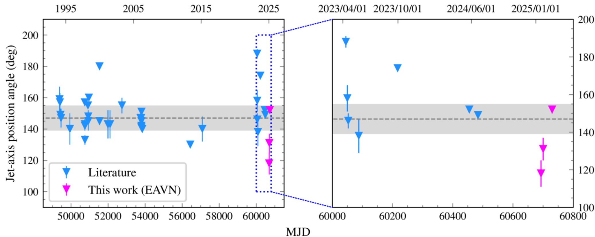
Figure 2. from Xi Yan et al 2026 Astrophys. J. Lett. 1006 doi:10.3847/2041-8213/ae80c8 https://dx.doi.org/10.3847/2041-8213/ae80c8 © 2026. The Author(s). Published by the American Astronomical Society.
