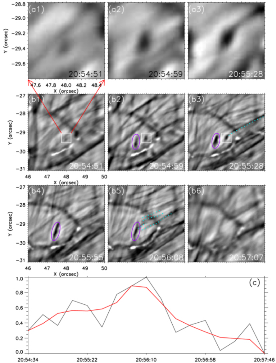
Figure 3. from Qifan Dong et al 2026 Astrophys. J. Lett. 1005 doi:10.3847/2041-8213/ae80be https://dx.doi.org/10.3847/2041-8213/ae80be © 2026. The Author(s). Published by the American Astronomical Society.
