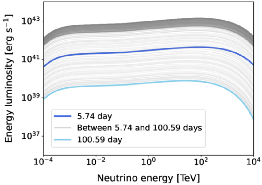
Figure 3. from Ryo Sawada et al 2026 Astrophys. J. Lett. 1005 doi:10.3847/2041-8213/ae80bd https://dx.doi.org/10.3847/2041-8213/ae80bd © 2026. The Author(s). Published by the American Astronomical Society.
