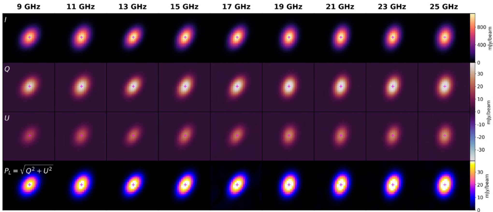
Figure 7. from Collin T. Christy et al 2026 Astrophys. J. Lett. 1006 doi:10.3847/2041-8213/ae80bc https://dx.doi.org/10.3847/2041-8213/ae80bc © 2026. The Author(s). Published by the American Astronomical Society.
