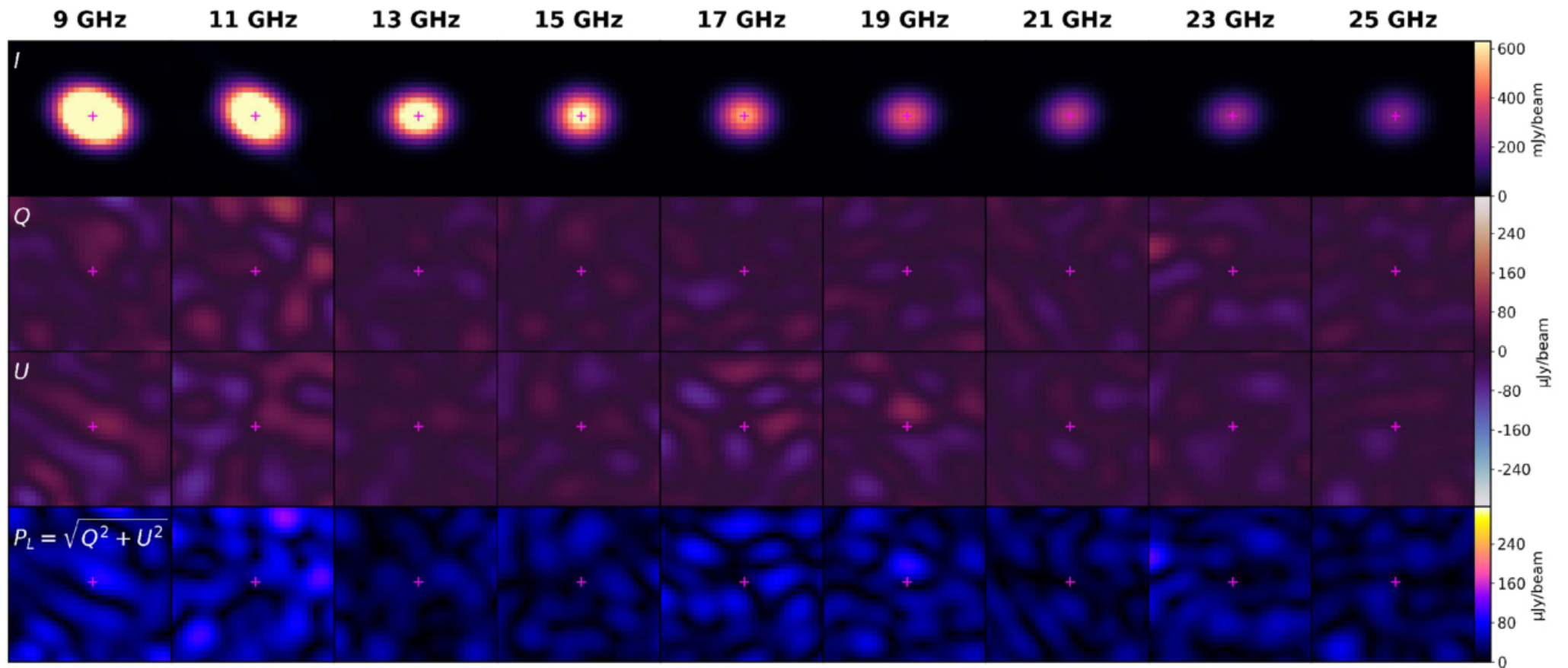
Figure 6. from Collin T. Christy et al 2026 Astrophys. J. Lett. 1006 doi:10.3847/2041-8213/ae80bc https://dx.doi.org/10.3847/2041-8213/ae80bc © 2026. The Author(s). Published by the American Astronomical Society.
