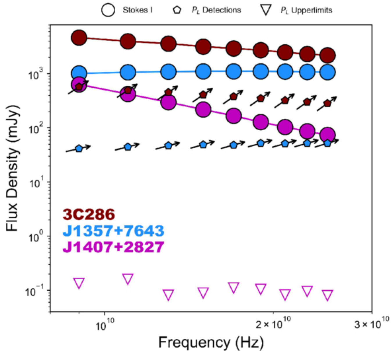
Figure 5. from Collin T. Christy et al 2026 Astrophys. J. Lett. 1006 doi:10.3847/2041-8213/ae80bc https://dx.doi.org/10.3847/2041-8213/ae80bc © 2026. The Author(s). Published by the American Astronomical Society.
