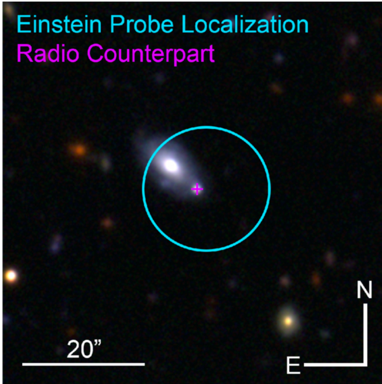
Figure 1. from Collin T. Christy et al 2026 Astrophys. J. Lett. 1006 doi:10.3847/2041-8213/ae80bc https://dx.doi.org/10.3847/2041-8213/ae80bc © 2026. The Author(s). Published by the American Astronomical Society.
