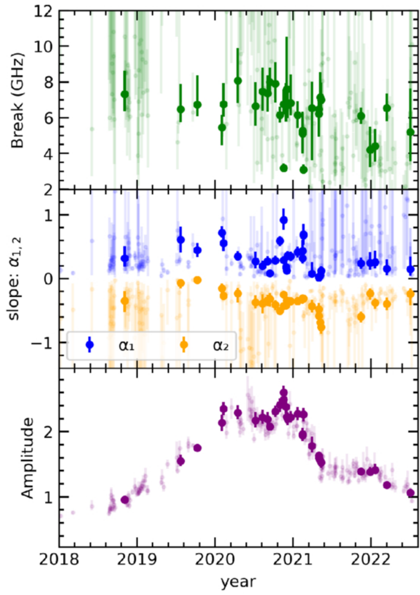
Figure 8. from S. I. Stathopoulos et al 2026 Astrophys. J. Lett. 1006 doi:10.3847/2041-8213/ae80bb https://dx.doi.org/10.3847/2041-8213/ae80bb © 2026. The Author(s). Published by the American Astronomical Society.
