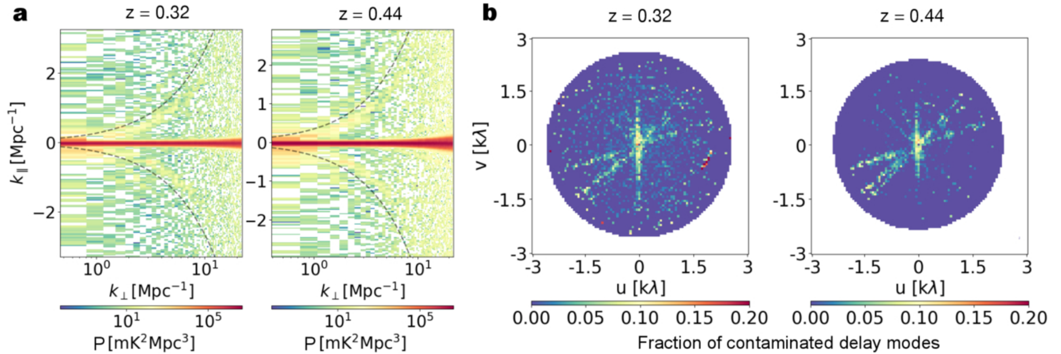
Figure 8. from Sourabh Paul et al 2026 Astrophys. J. Lett. 1005 doi:10.3847/2041-8213/ae808f https://dx.doi.org/10.3847/2041-8213/ae808f © 2026. The Author(s). Published by the American Astronomical Society.
