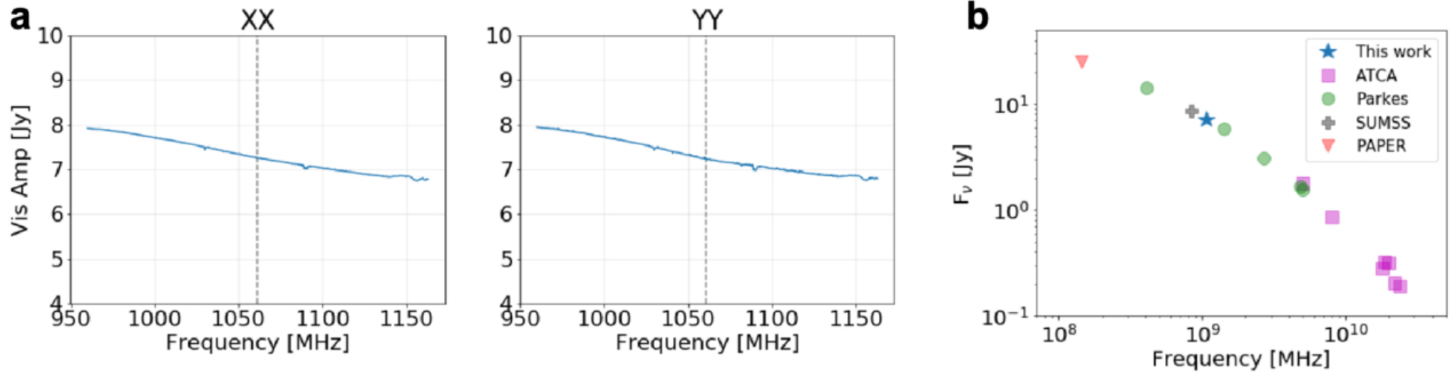
Figure 2. from Sourabh Paul et al 2026 Astrophys. J. Lett. 1005 doi:10.3847/2041-8213/ae808f https://dx.doi.org/10.3847/2041-8213/ae808f © 2026. The Author(s). Published by the American Astronomical Society.
