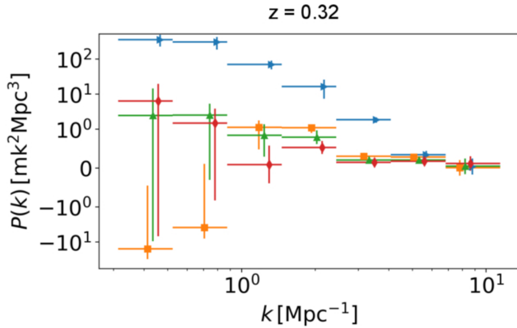
Figure 13. from Sourabh Paul et al 2026 Astrophys. J. Lett. 1005 doi:10.3847/2041-8213/ae808f https://dx.doi.org/10.3847/2041-8213/ae808f © 2026. The Author(s). Published by the American Astronomical Society.
