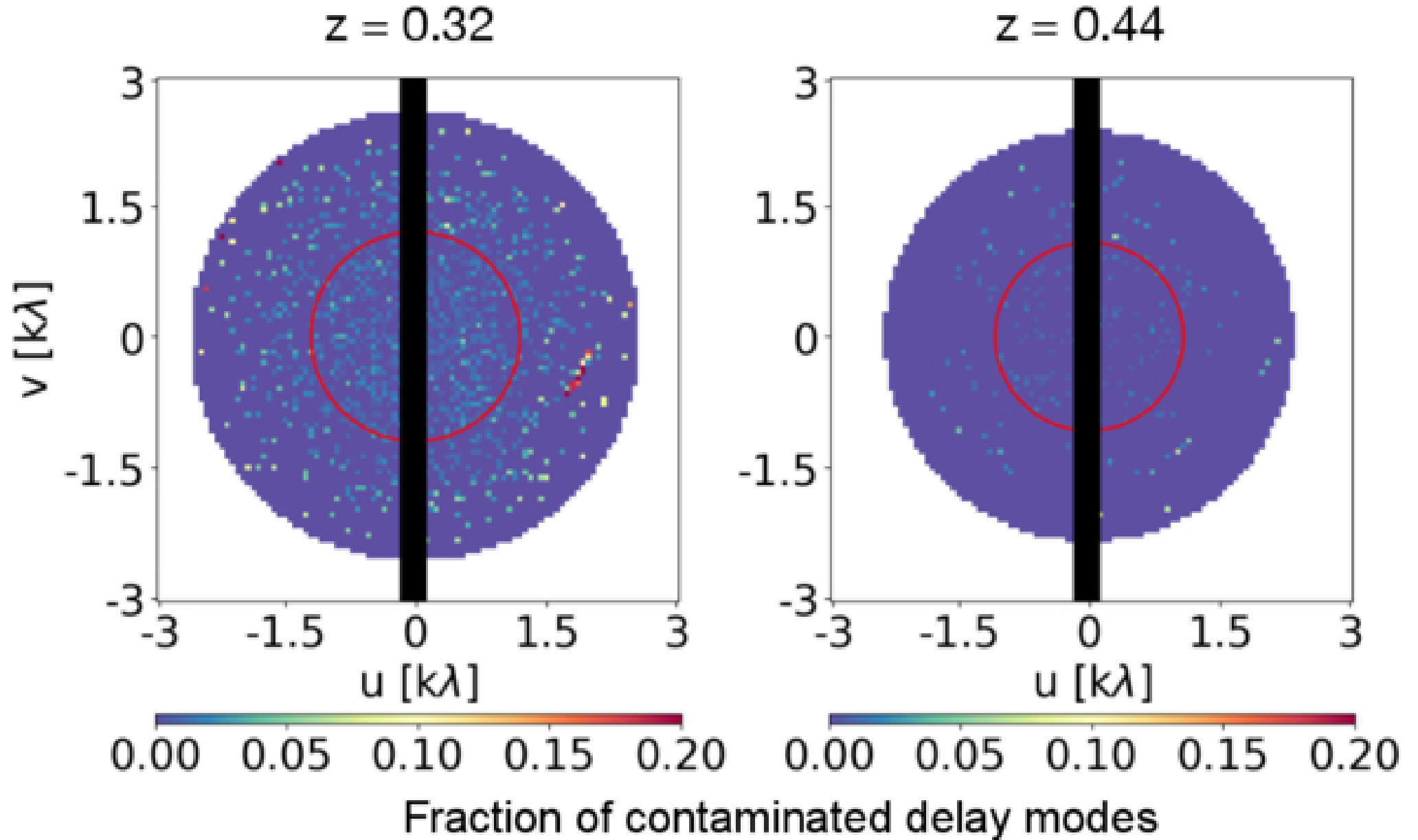
Figure 11. from Sourabh Paul et al 2026 Astrophys. J. Lett. 1005 doi:10.3847/2041-8213/ae808f https://dx.doi.org/10.3847/2041-8213/ae808f © 2026. The Author(s). Published by the American Astronomical Society.
