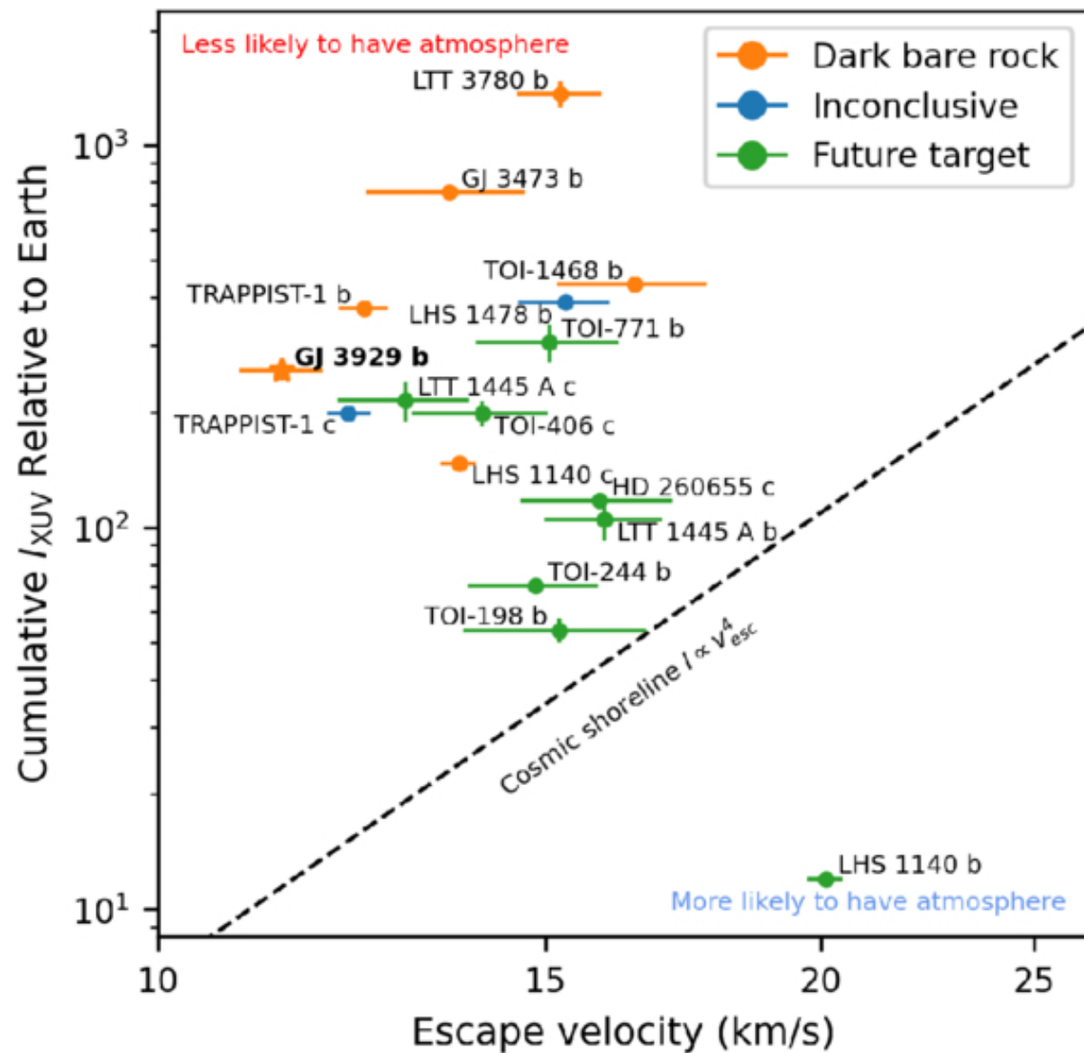
Figure 9. from Nicholas J. Connors et al 2026 Astrophys. J. Lett. 1006 doi:10.3847/2041-8213/ae8018 https://dx.doi.org/10.3847/2041-8213/ae8018 © 2026. The Author(s). Published by the American Astronomical Society.
