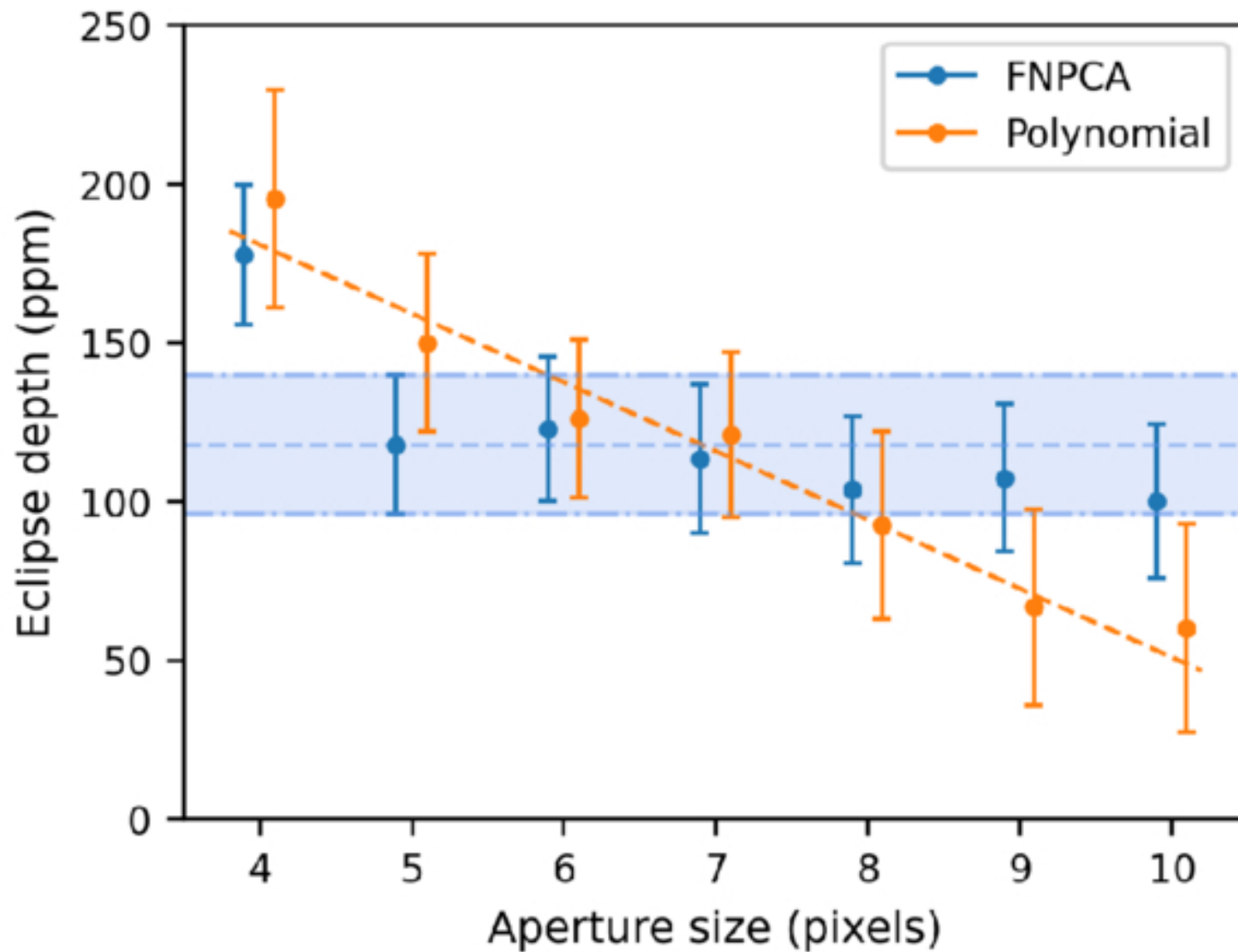
Figure 6. from Nicholas J. Connors et al 2026 Astrophys. J. Lett. 1006 doi:10.3847/2041-8213/ae8018 https://dx.doi.org/10.3847/2041-8213/ae8018 © 2026. The Author(s). Published by the American Astronomical Society.
