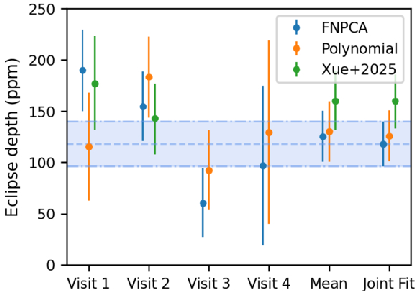
Figure 4. from Nicholas J. Connors et al 2026 Astrophys. J. Lett. 1006 doi:10.3847/2041-8213/ae8018 https://dx.doi.org/10.3847/2041-8213/ae8018 © 2026. The Author(s). Published by the American Astronomical Society.
