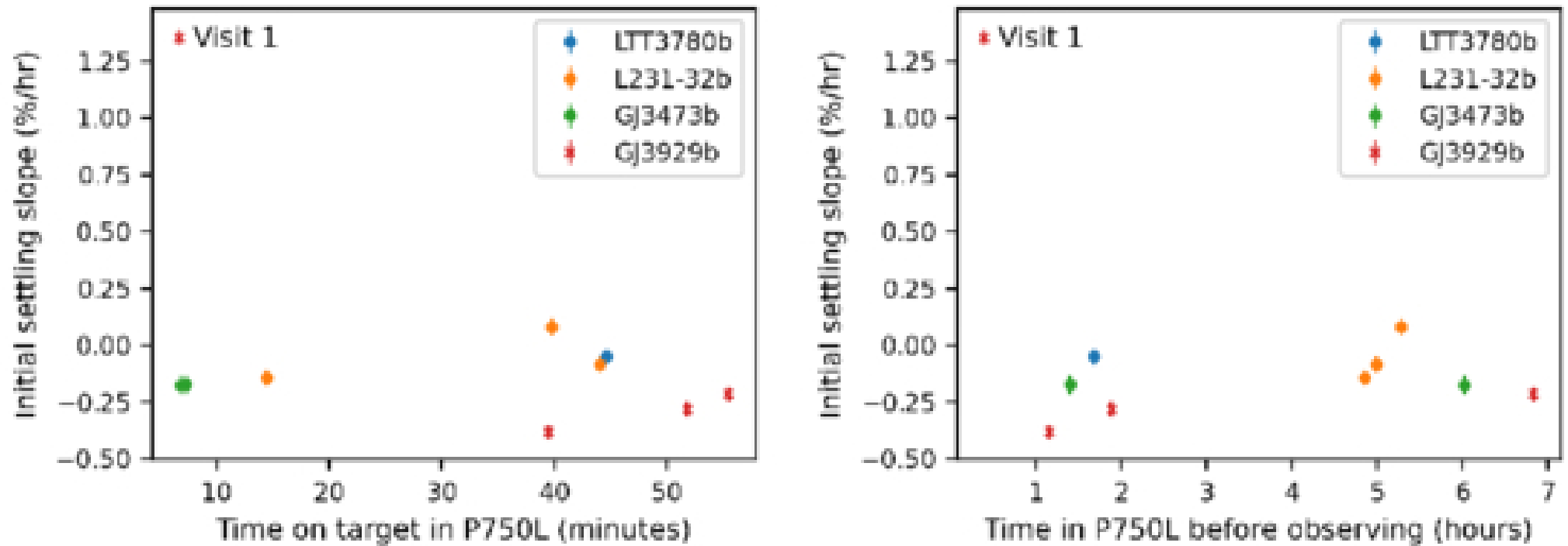
Figure 14. from Nicholas J. Connors et al 2026 Astrophys. J. Lett. 1006 doi:10.3847/2041-8213/ae8018 https://dx.doi.org/10.3847/2041-8213/ae8018 © 2026. The Author(s). Published by the American Astronomical Society.
