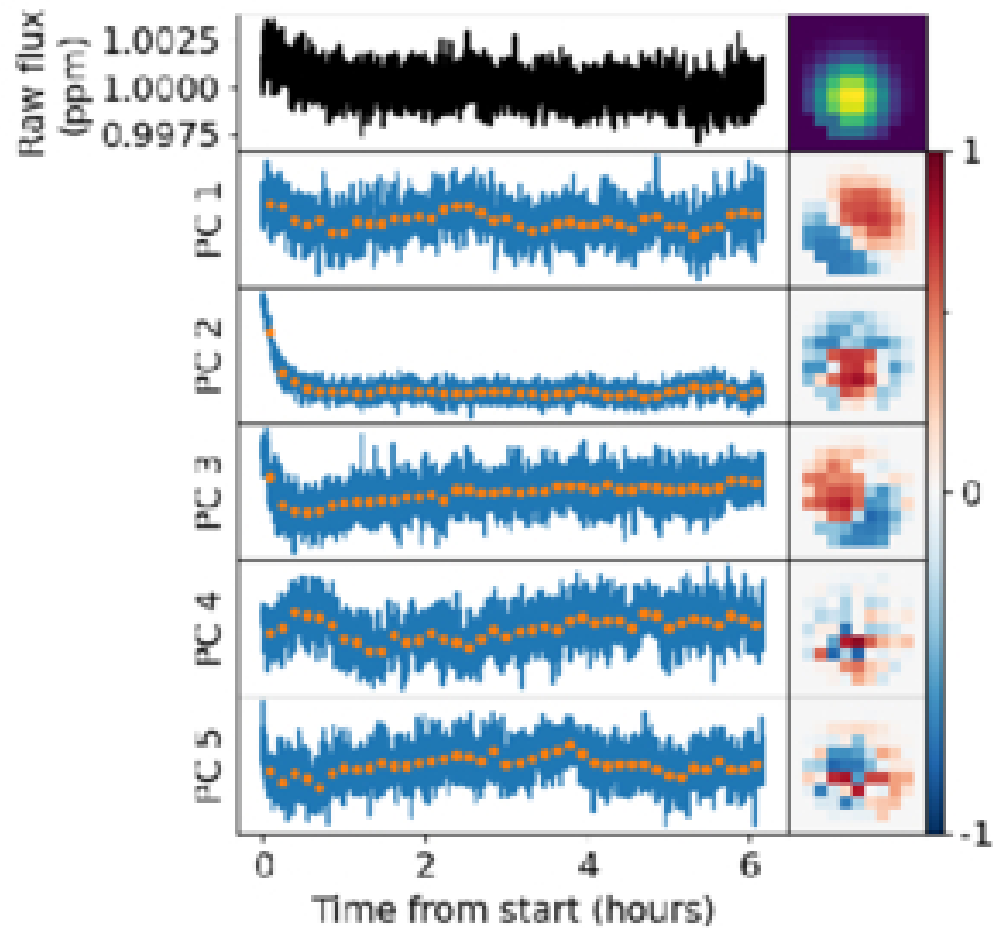
Figure 12. from Nicholas J. Connors et al 2026 Astrophys. J. Lett. 1006 doi:10.3847/2041-8213/ae8018 https://dx.doi.org/10.3847/2041-8213/ae8018 © 2026. The Author(s). Published by the American Astronomical Society.
