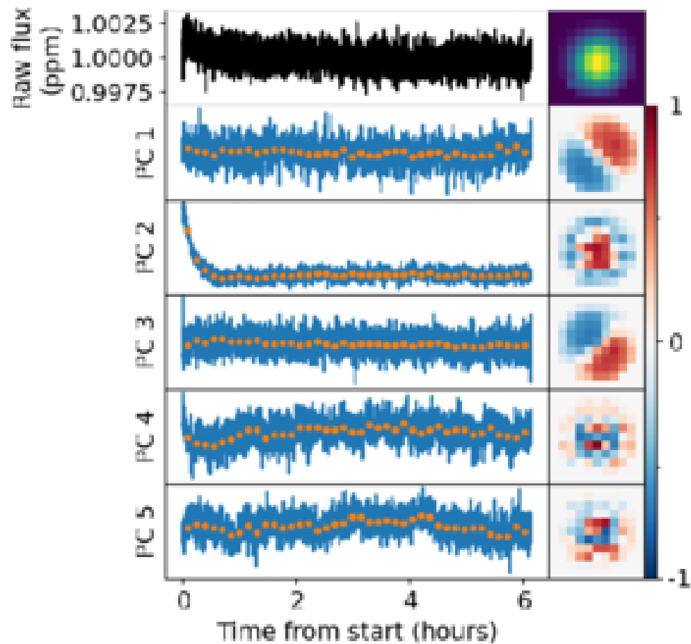
Figure 11. from Nicholas J. Connors et al 2026 Astrophys. J. Lett. 1006 doi:10.3847/2041-8213/ae8018 https://dx.doi.org/10.3847/2041-8213/ae8018 © 2026. The Author(s). Published by the American Astronomical Society.
