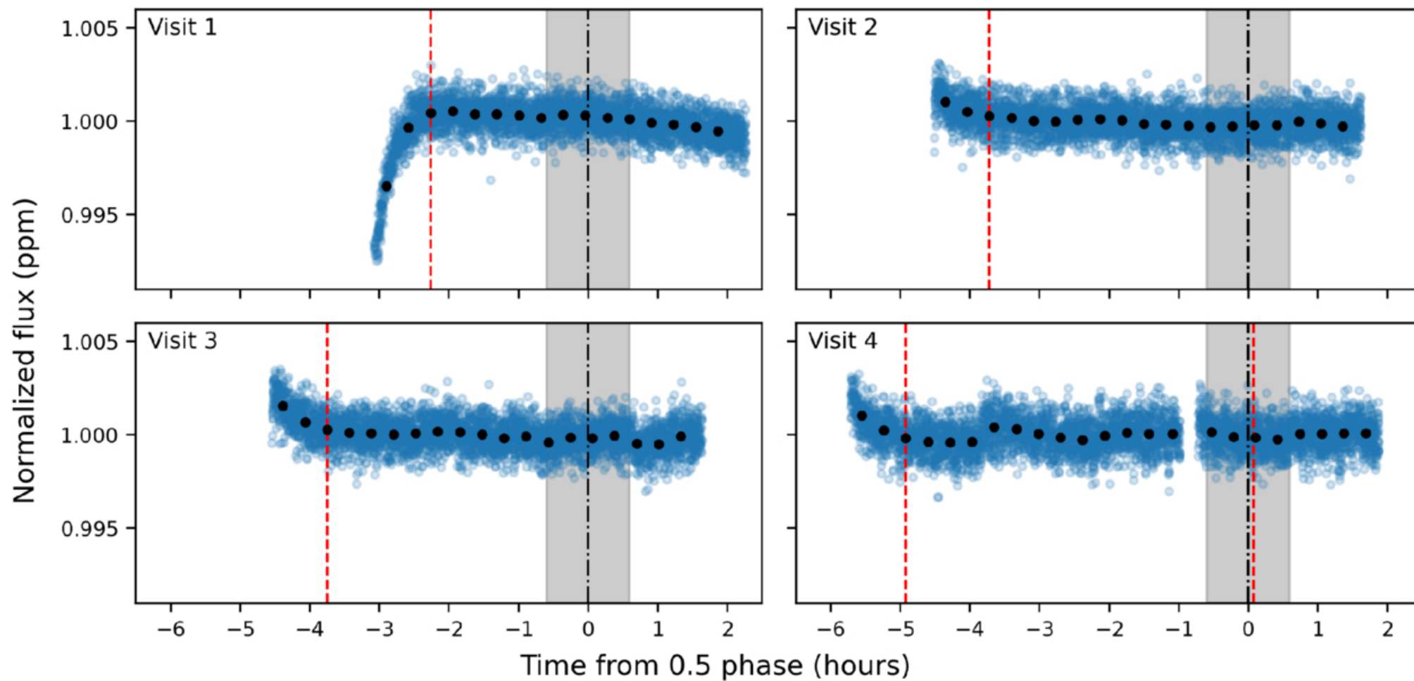
Figure 1. from Nicholas J. Connors et al 2026 Astrophys. J. Lett. 1006 doi:10.3847/2041-8213/ae8018 https://dx.doi.org/10.3847/2041-8213/ae8018 © 2026. The Author(s). Published by the American Astronomical Society.
