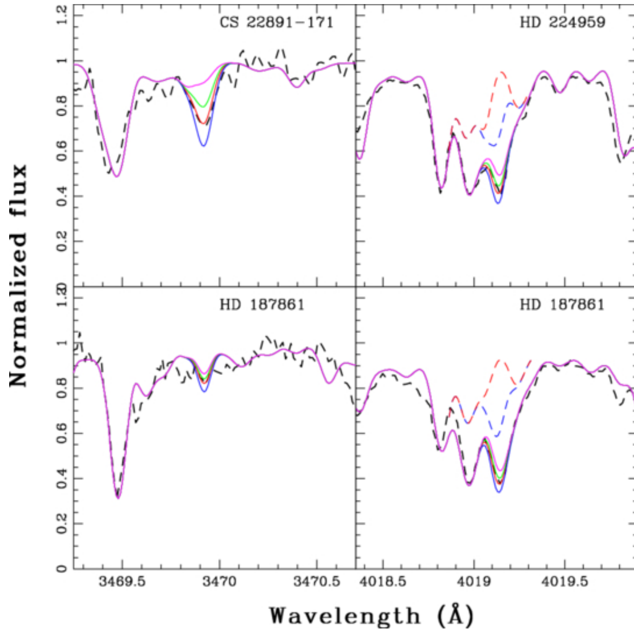
Figure 3. from A. M. Riyas et al 2026 Astrophys. J. Lett. 1006 doi:10.3847/2041-8213/ae8013 https://dx.doi.org/10.3847/2041-8213/ae8013 © 2026. The Author(s). Published by the American Astronomical Society.
