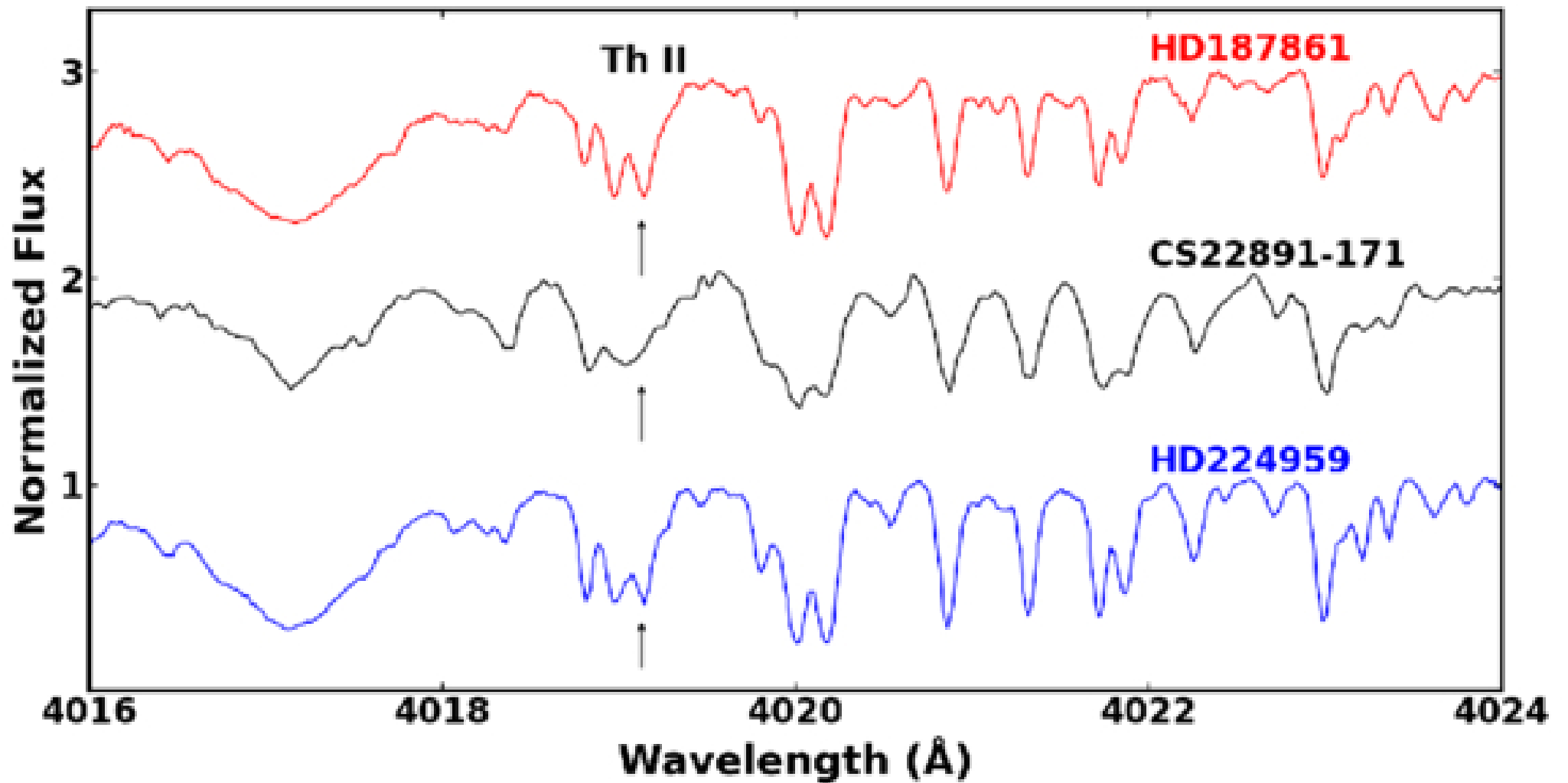
Figure 2. from A. M. Riyas et al 2026 Astrophys. J. Lett. 1006 doi:10.3847/2041-8213/ae8013 https://dx.doi.org/10.3847/2041-8213/ae8013 © 2026. The Author(s). Published by the American Astronomical Society.
