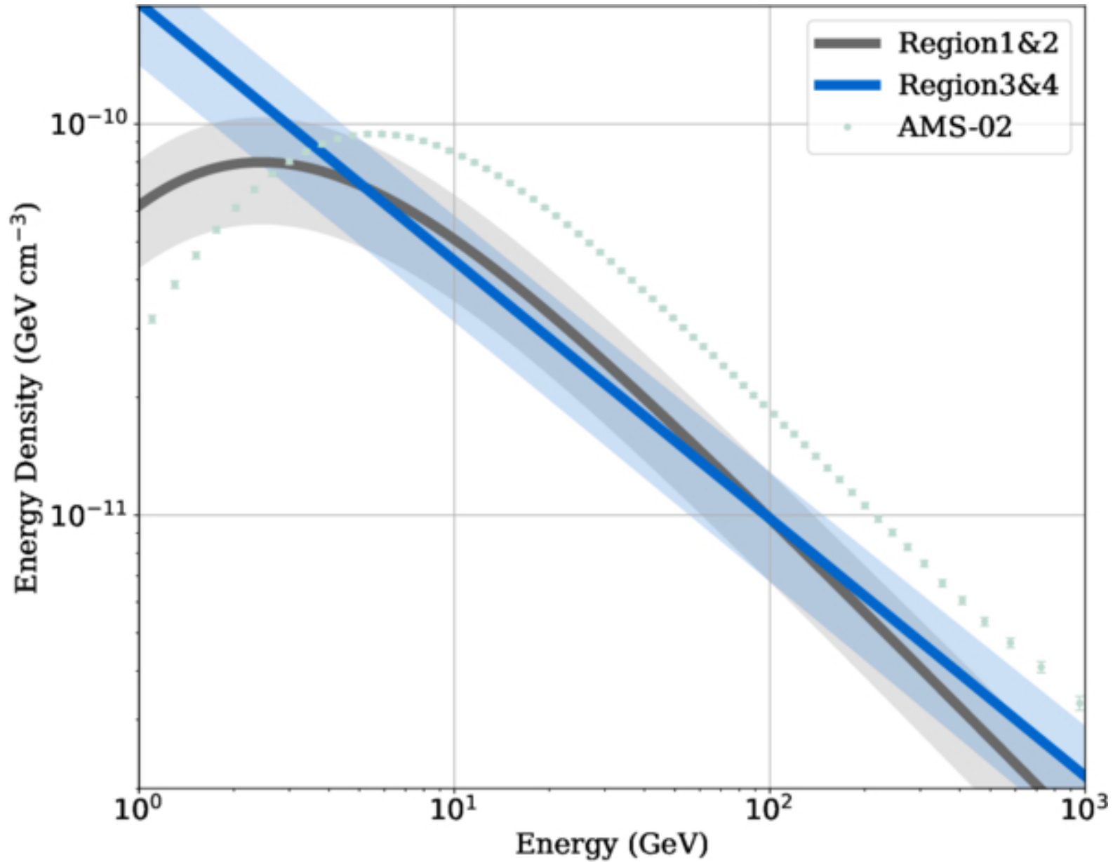
Figure 8. from Ningyu Tang et al 2026 Astrophys. J. Lett. 1005 doi:10.3847/2041-8213/ae8010 https://dx.doi.org/10.3847/2041-8213/ae8010 © 2026. The Author(s). Published by the American Astronomical Society.
