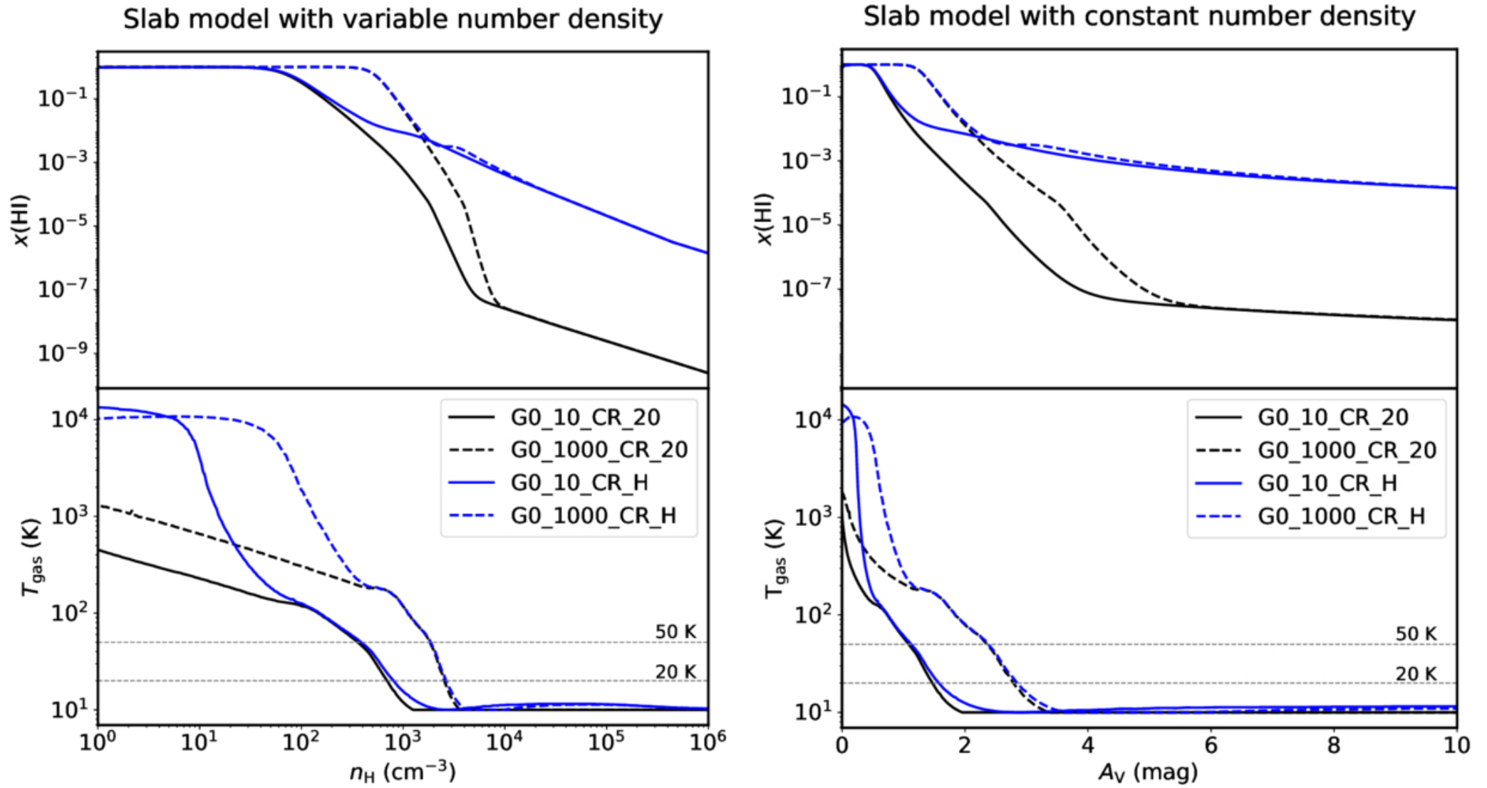
Figure 7. from Ningyu Tang et al 2026 Astrophys. J. Lett. 1005 doi:10.3847/2041-8213/ae8010 https://dx.doi.org/10.3847/2041-8213/ae8010 © 2026. The Author(s). Published by the American Astronomical Society.
