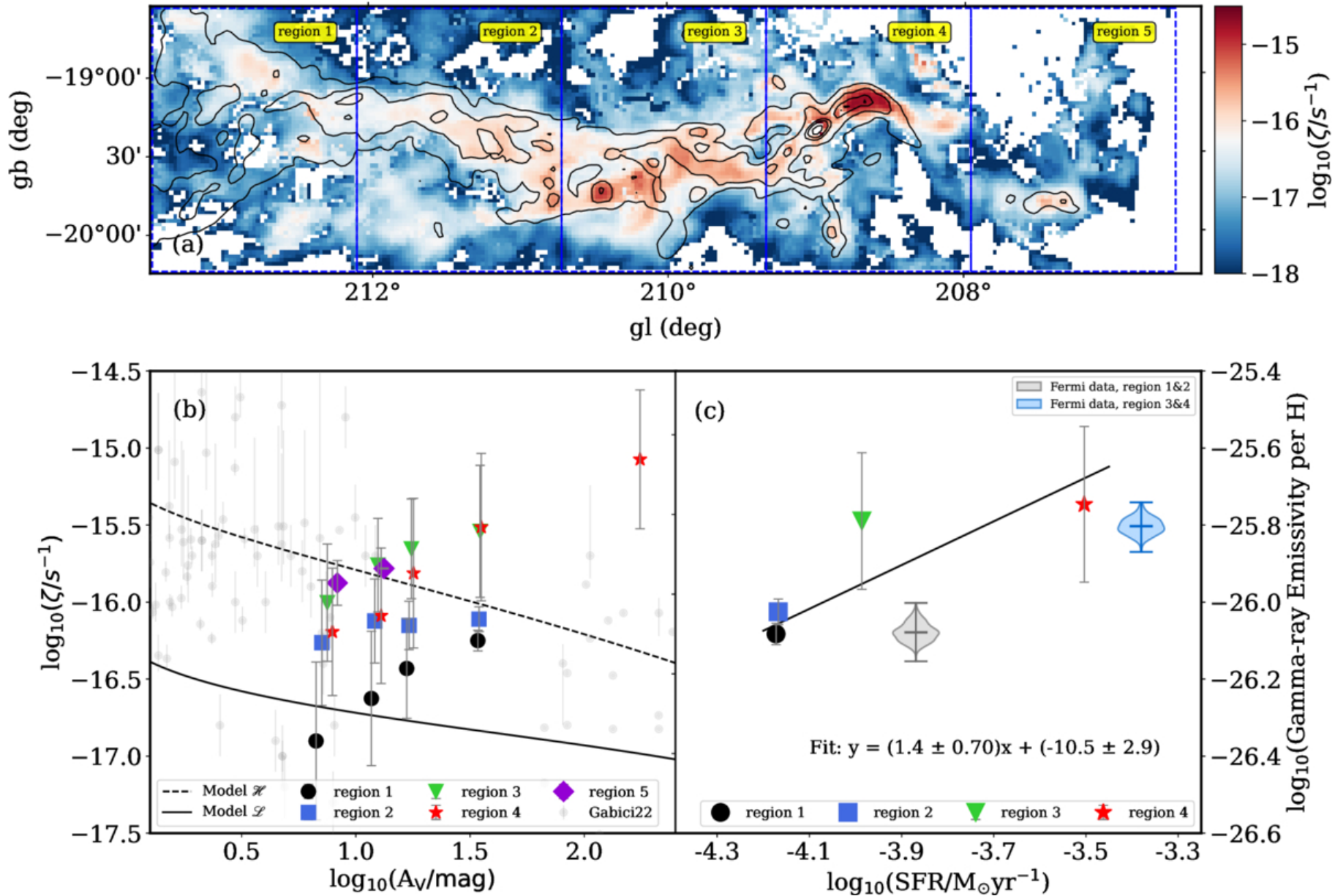
Figure 4. from Ningyu Tang et al 2026 Astrophys. J. Lett. 1005 doi:10.3847/2041-8213/ae8010 https://dx.doi.org/10.3847/2041-8213/ae8010 © 2026. The Author(s). Published by the American Astronomical Society.
