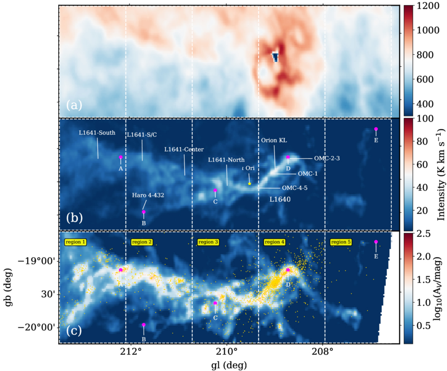
Figure 1. from Ningyu Tang et al 2026 Astrophys. J. Lett. 1005 doi:10.3847/2041-8213/ae8010 https://dx.doi.org/10.3847/2041-8213/ae8010 © 2026. The Author(s). Published by the American Astronomical Society.
