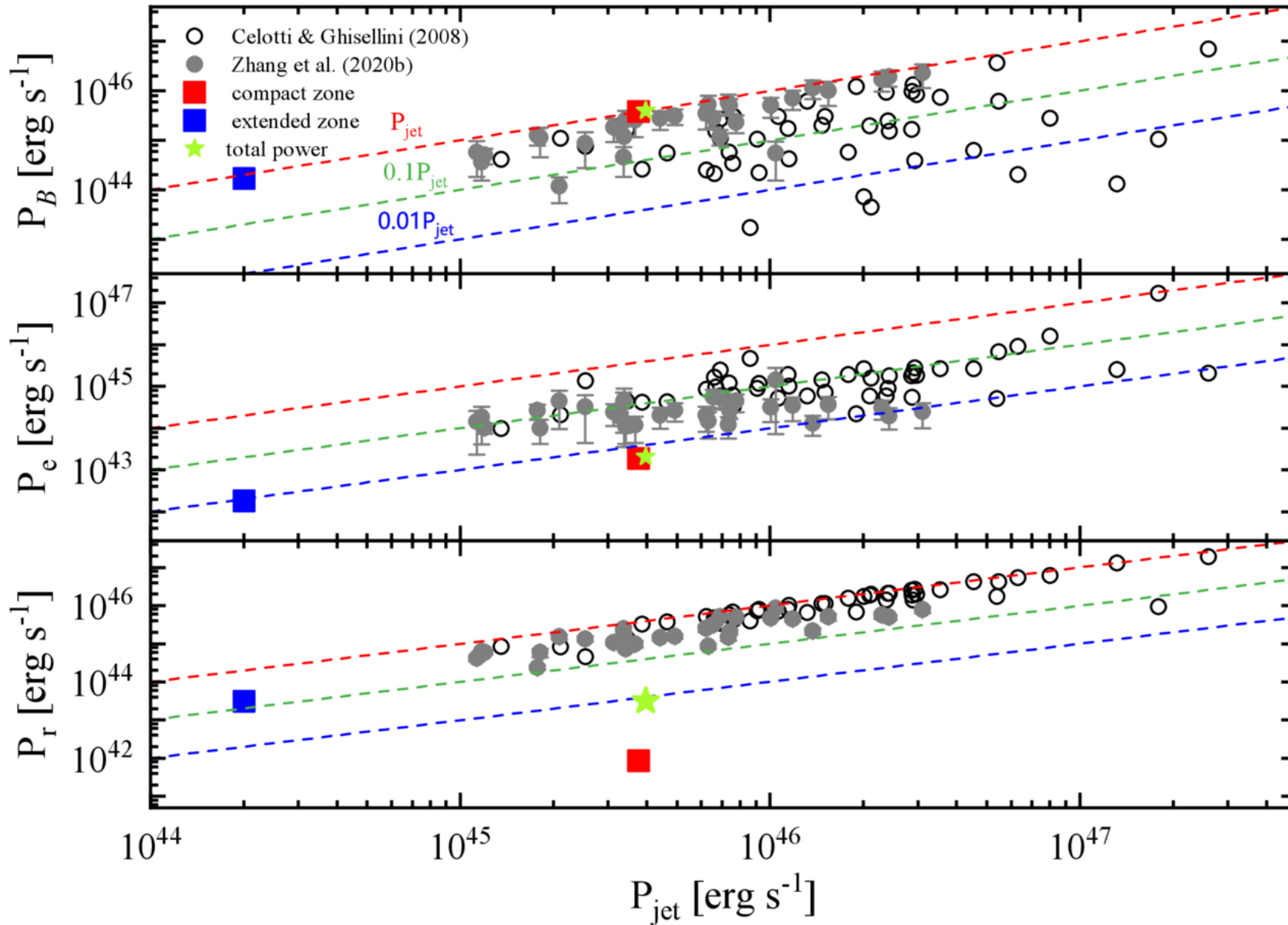
Figure 8. from Shuo-Yu Liu et al 2026 Astrophys. J. Lett. 1005 doi:10.3847/2041-8213/ae800e https://dx.doi.org/10.3847/2041-8213/ae800e © 2026. The Author(s). Published by the American Astronomical Society.
