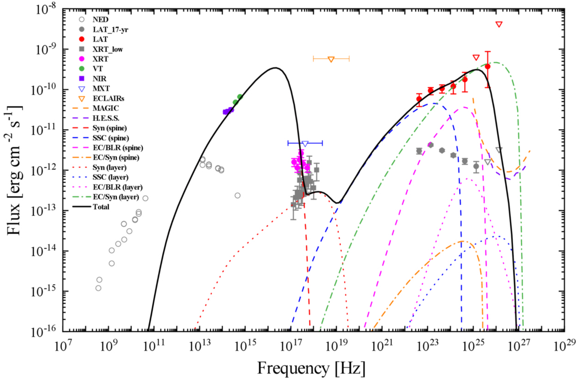
Figure 6. from Shuo-Yu Liu et al 2026 Astrophys. J. Lett. 1005 doi:10.3847/2041-8213/ae800e https://dx.doi.org/10.3847/2041-8213/ae800e © 2026. The Author(s). Published by the American Astronomical Society.
