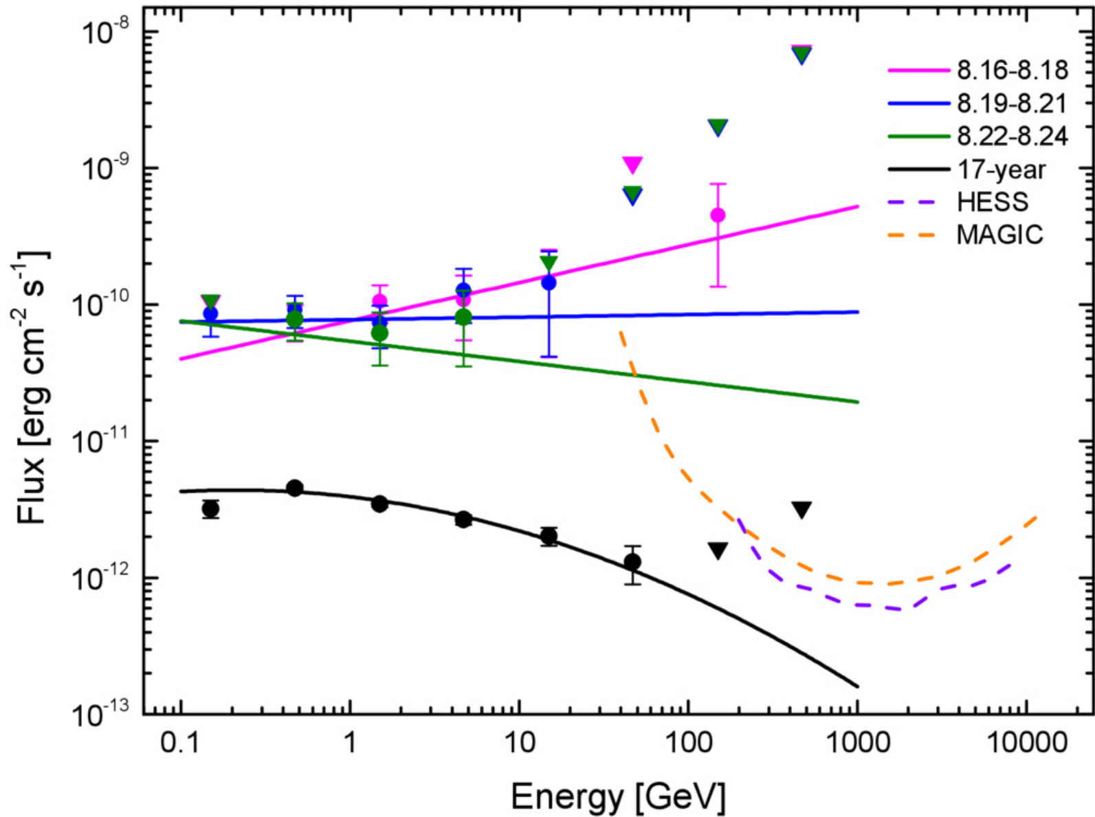
Figure 5. from Shuo-Yu Liu et al 2026 Astrophys. J. Lett. 1005 doi:10.3847/2041-8213/ae800e https://dx.doi.org/10.3847/2041-8213/ae800e © 2026. The Author(s). Published by the American Astronomical Society.
