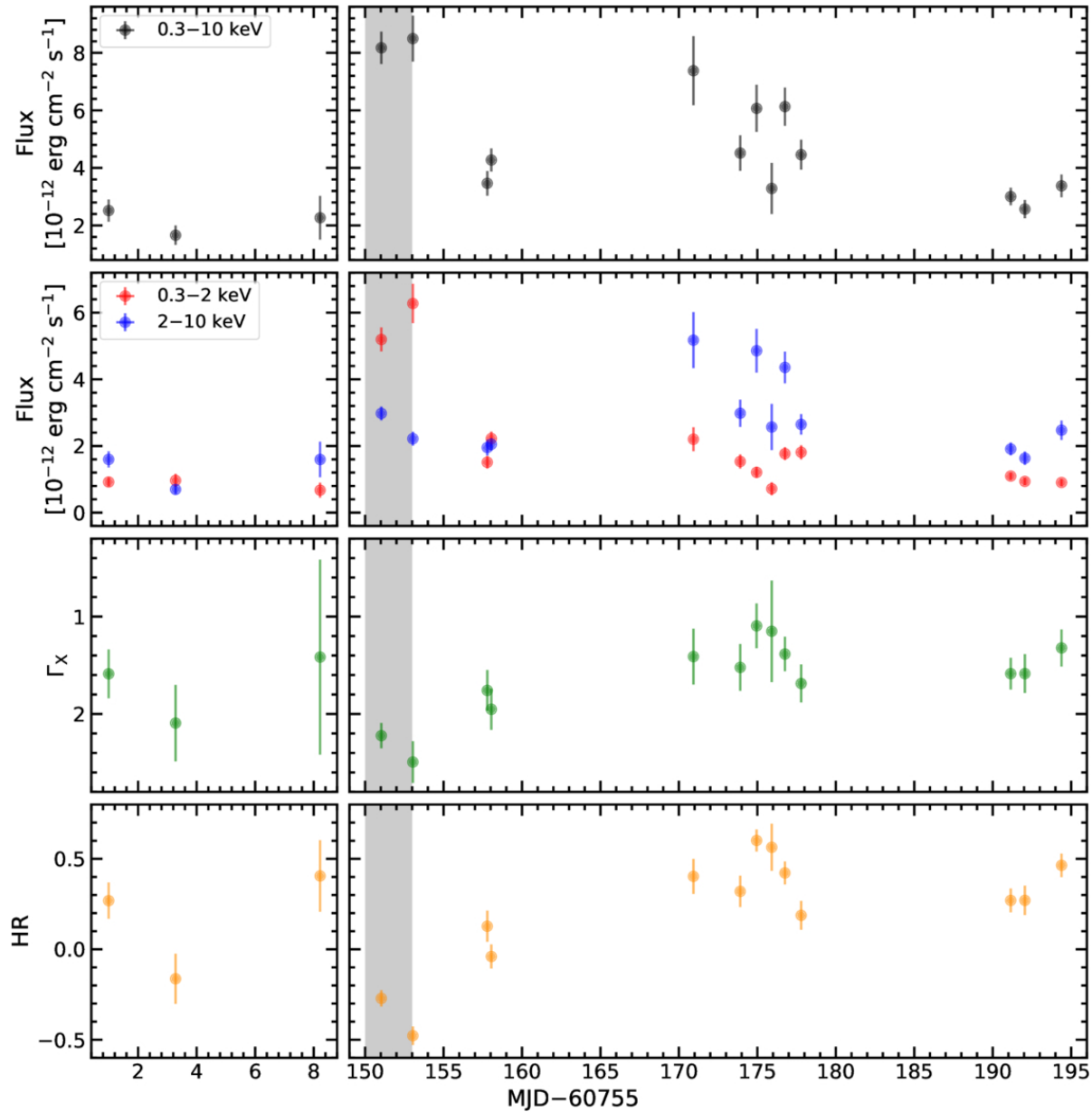
Figure 4. from Shuo-Yu Liu et al 2026 Astrophys. J. Lett. 1005 doi:10.3847/2041-8213/ae800e https://dx.doi.org/10.3847/2041-8213/ae800e © 2026. The Author(s). Published by the American Astronomical Society.
