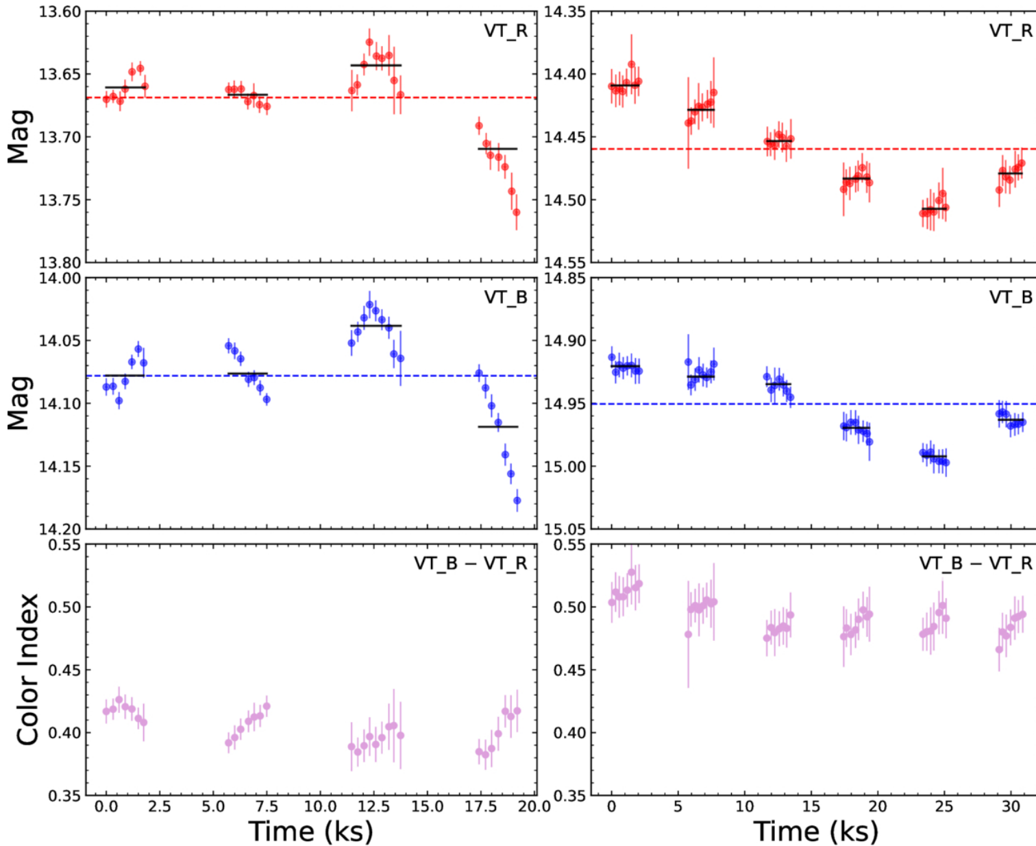
Figure 2. from Shuo-Yu Liu et al 2026 Astrophys. J. Lett. 1005 doi:10.3847/2041-8213/ae800e https://dx.doi.org/10.3847/2041-8213/ae800e © 2026. The Author(s). Published by the American Astronomical Society.
